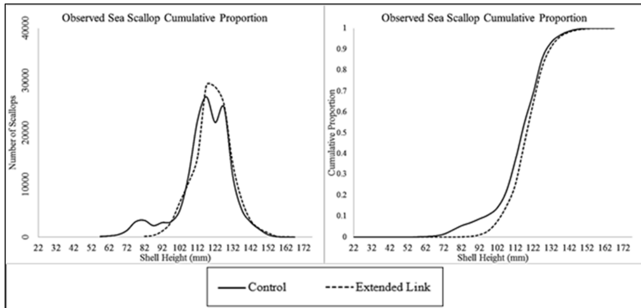
Figure 7: The pooled scallop shell height frequency distribution and cumulative proportion curves for the control dredge (solid line) and the extended link apron (dashed line) for the FV Diligence cruise).
