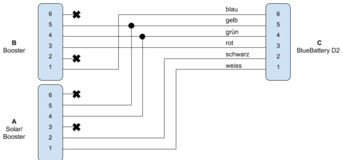
Y-Adapter (Solar/Booster)
