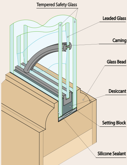
Cross Section at Insulated Leaded Glass
