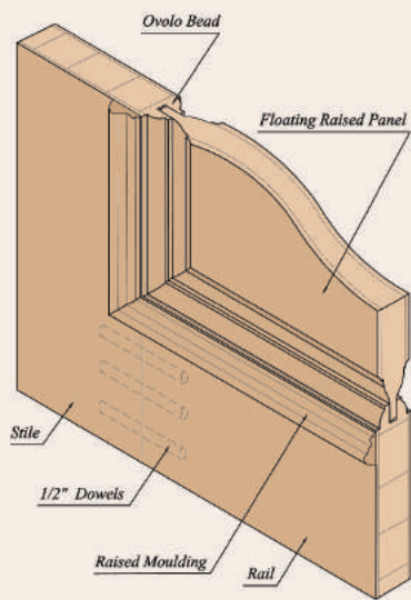
Mahogany Cross Section
