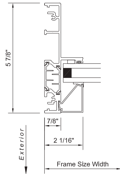
series 7675 direct set window jamb - equal leg block frame
