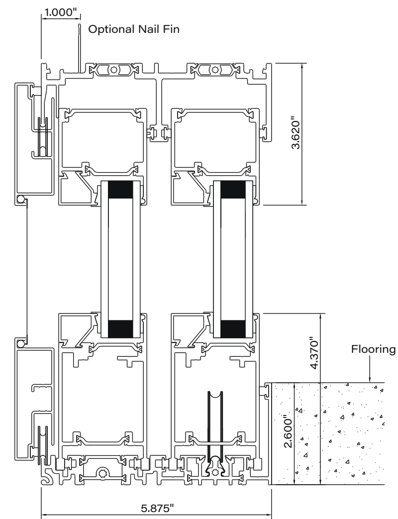
7650 2.6" water barrier sill
