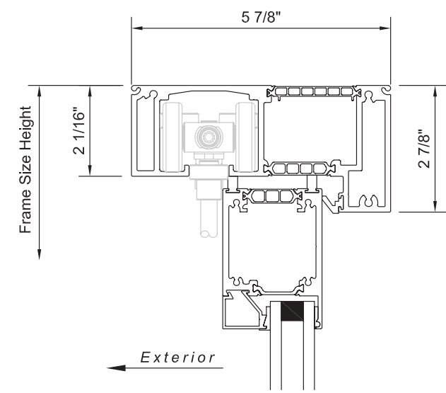
head load bi-fold fold-out head
