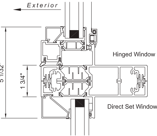
series 7660, 7670 hinged window and 7675 direct set window horizontal mull
