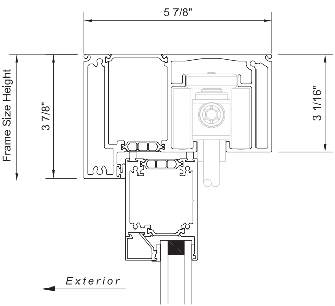
heavy-duty head load bi-fold fold-in head
