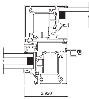
interlock condition
