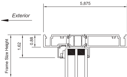
head equal leg frame triple pane
