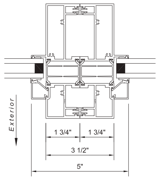
3 1/2" vertical mull
