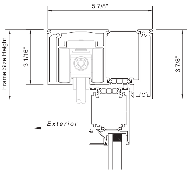
heavy-duty head load bi-fold fold-out head
