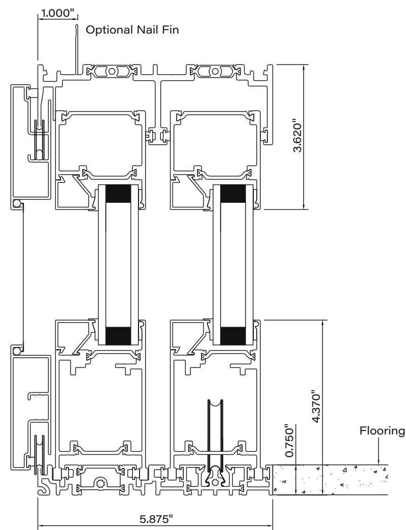
7650 flush sill
