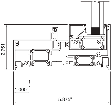
nail-fin condition
