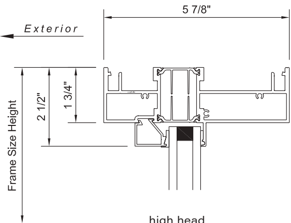
high head equal leg block frame
