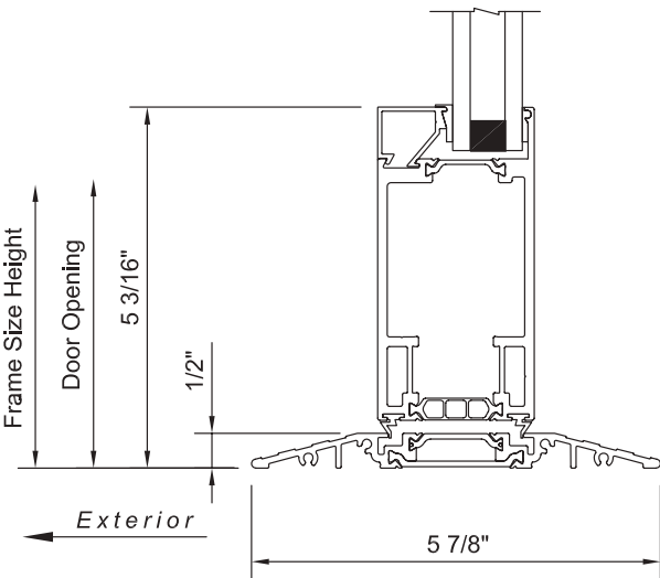
threshold
