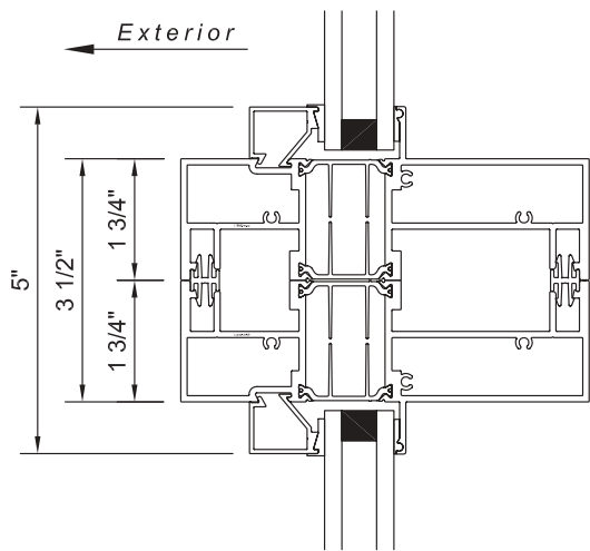
3 1/2" horizontal mull
