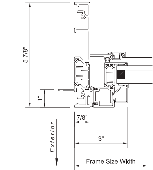
series 7660 awning and series 7670 casement window jamb - nail fin frame
