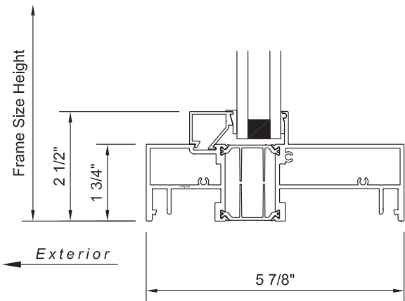
high sill equal leg block frame
