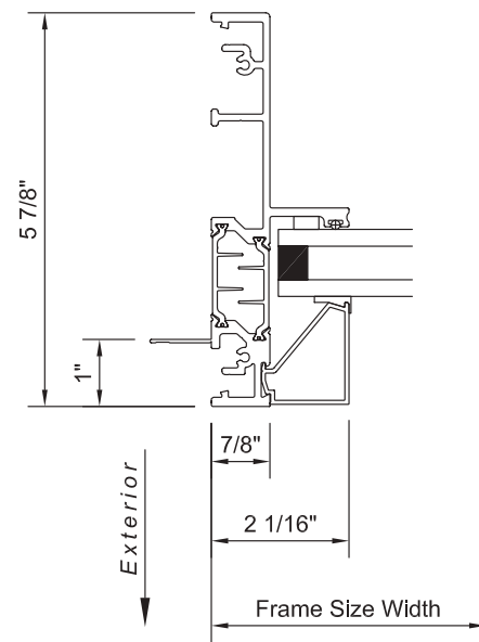
series 7675 direct set window jamb - nail fin frame
