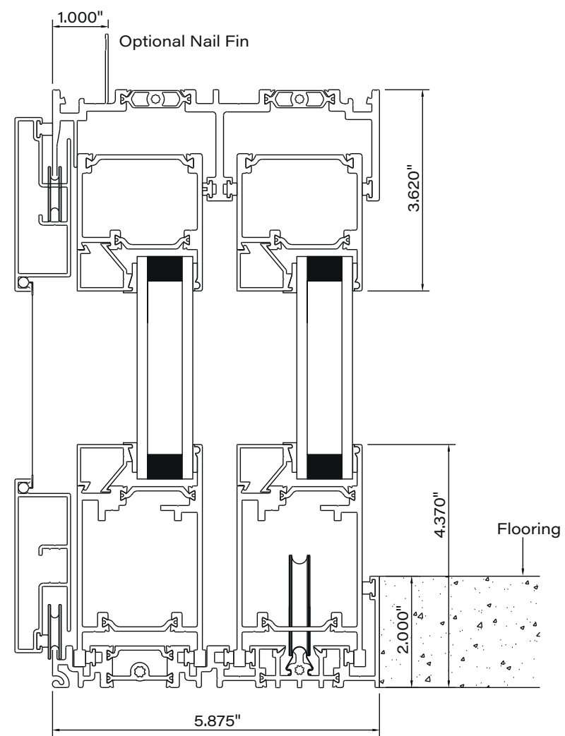
7650 2" water barrier sill
