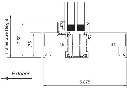
high sill equal leg frame triple pane
