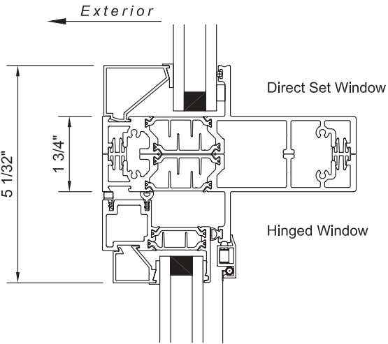
series 7660, 7670 hinged window and 7675 direct set window horizontal mull
