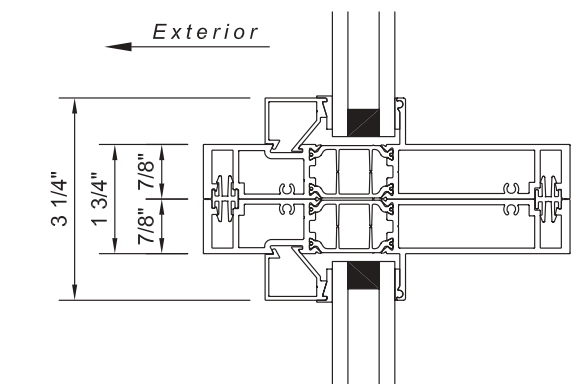
1 3/4" horizontal mull
