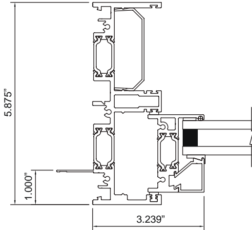
fixed panel
