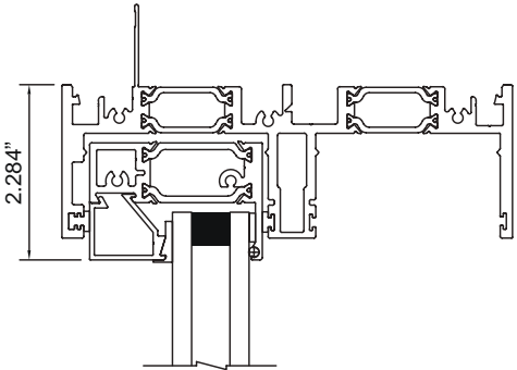
nail-fin condition
