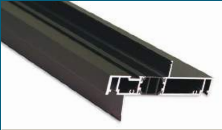
Extruded Nail Fin
