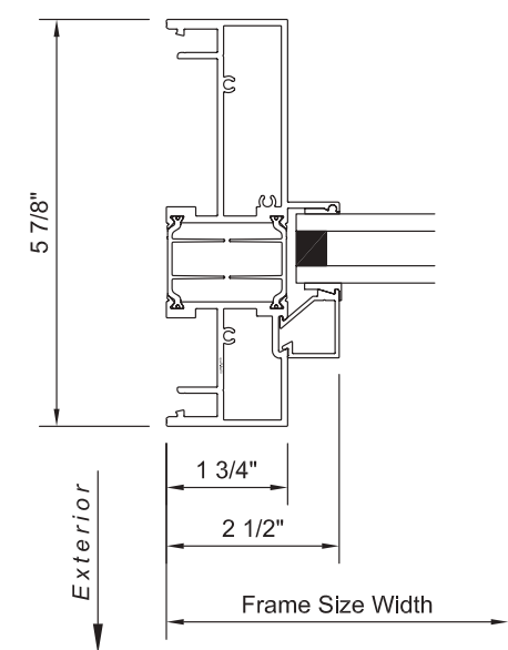
high jamb equal leg block frame
