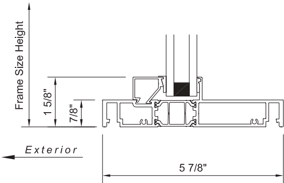
sill equal leg block frame
