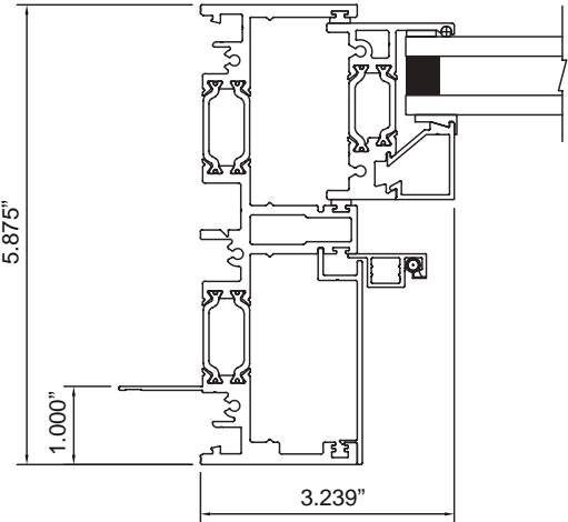
vent panel
