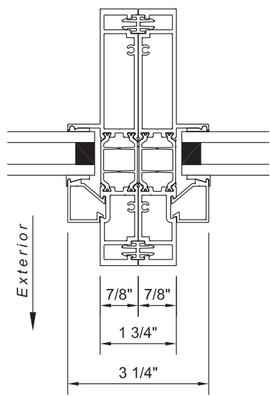
1 3/4" vertical mull
