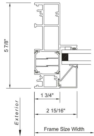
series 7675 direct set window jamb - equal leg block high frame
