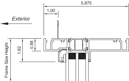
head nail fin frame triple pane
