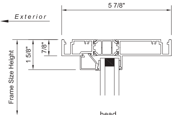
head equal leg block frame
