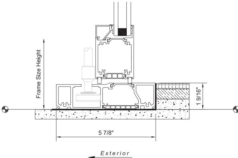
heavy-duty head load bi-fold fold-out with flush threshold
