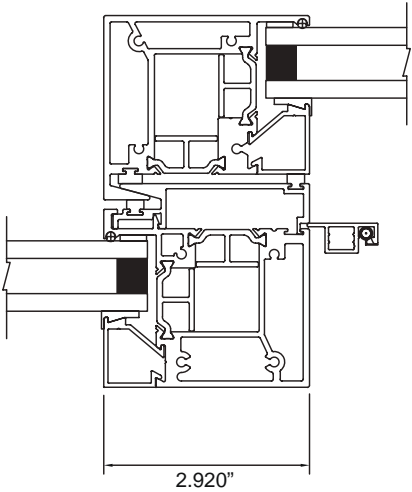
interlock condition
