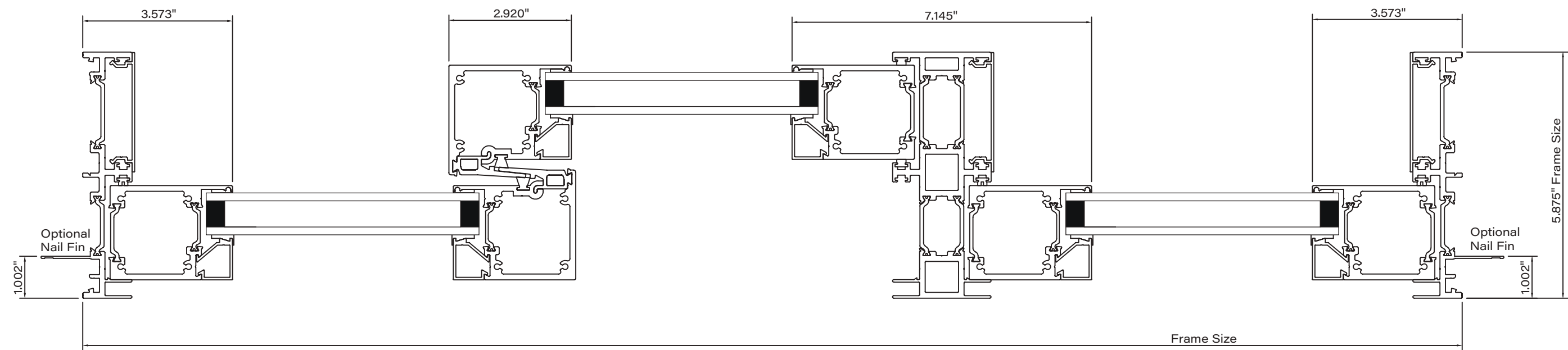
7650 OXO condition
