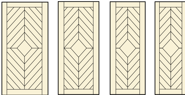
4'0" wide x 8'0" tall 3'6" wide x 8'0" tall 3'0" wide x 8'0" tall 2'8" wide x 8'0" tall
