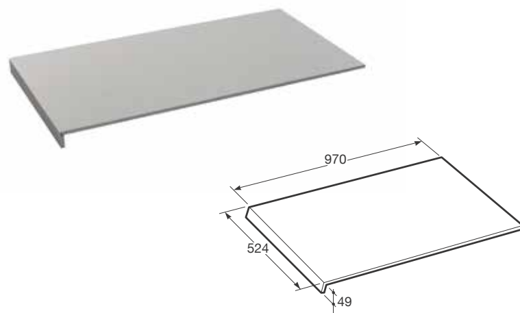
L4 OFF-WHITE LATTICE R 4,9 x 97.
