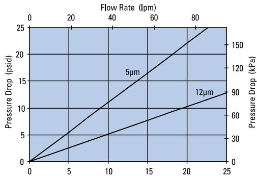
HPK02 8" DT Filter Only DT-9021-8, 8"/203mm
