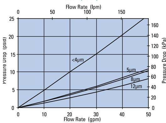
HPK04 16" DX2 Filter Only DX2-9600-16, 16.81"/427mm
