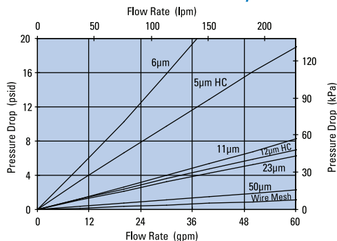
HPK03 8" Standard Filter Only
