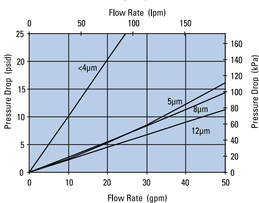
FPK04 8" DX2 Filter Only DX2-9600-8, 8.22"/208.8mm
