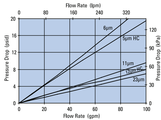
FPK04 13" Standard Filter Only
