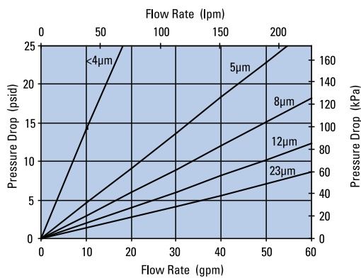
FPK04 4" DT Filter Only
