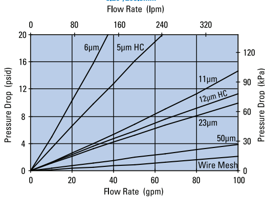
FPK04 8" Standard Filter Only
