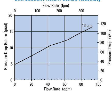
SRK Suction / Return Combo Assembly
