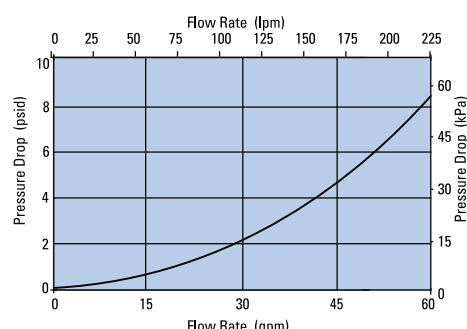
W023 Head Only
