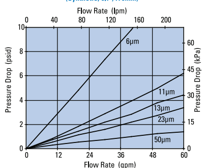
W023 Filter Only (Synthetic, 6.7"/170mm)
