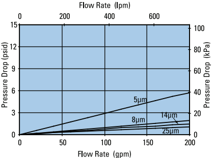
WL16 27" DT Filter Only
