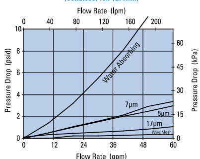
W023 Filter Only (Cellulose, 10.7"/271mm)
