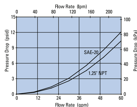
HBK05 Head Only
