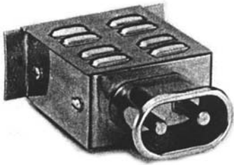
KA220 90 x 56 x 32 mm
