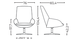
Aluminium round base Base redonda de aluminio
