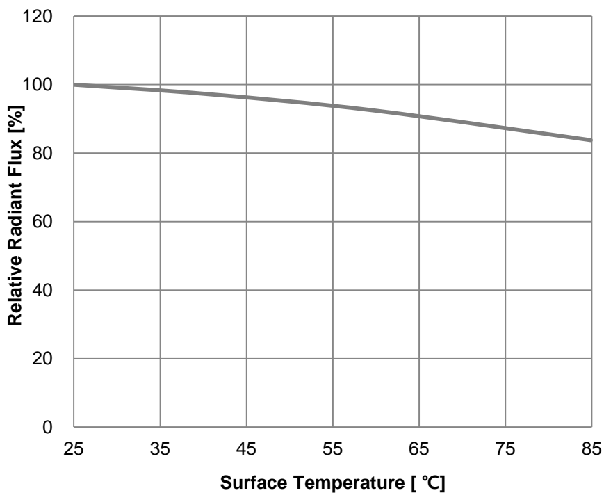
Fig 5. Surface Temperature vs. Relative Radiant Flux, I_F=1A
