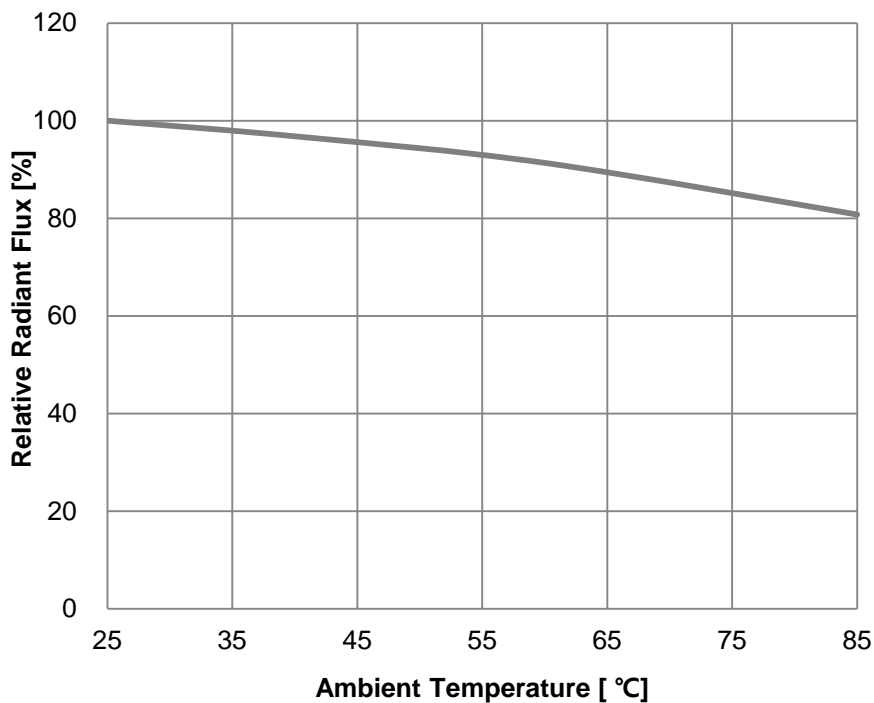
Fig 5. Ambient Temperature vs. Relative Radiant Flux, I_F=100\text{mA}
