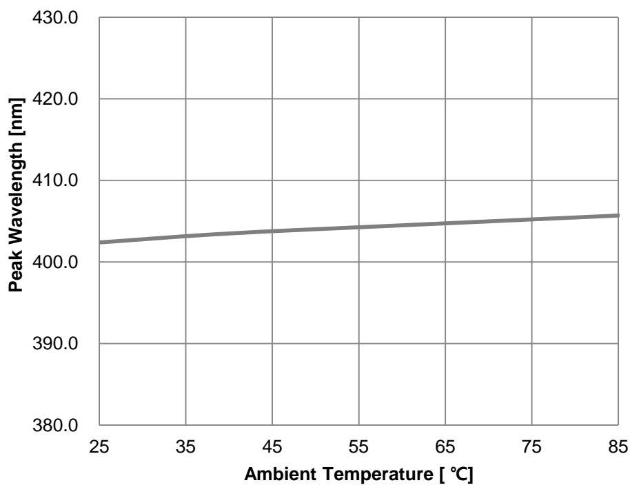
Fig 6. Ambient Temperature vs. Peak Wavelength, I_F=100\text{mA}
