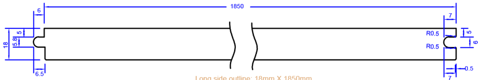
Long side outline: 18mm X 1850mm
