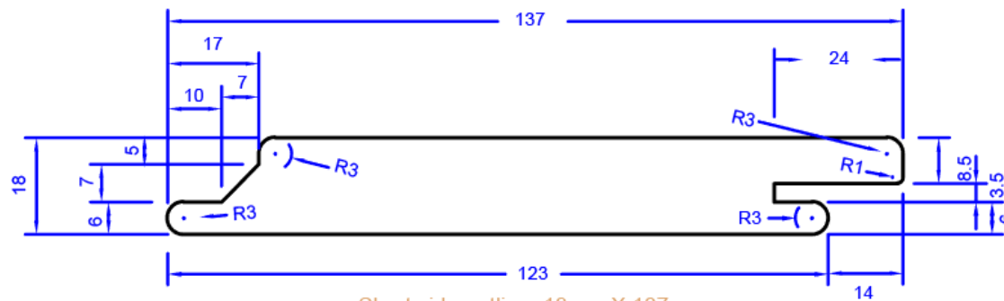
Short side outline: 18mm X 137mm
