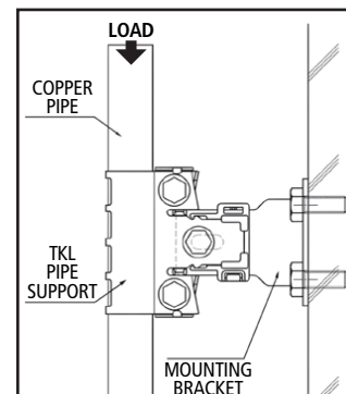
(Figure 6) Load Capacity
