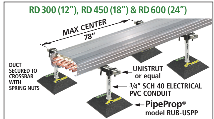
(Section 4) Pipe Prop RUB-USPP Configurations for Support of RD Series Lineset Ducting System
