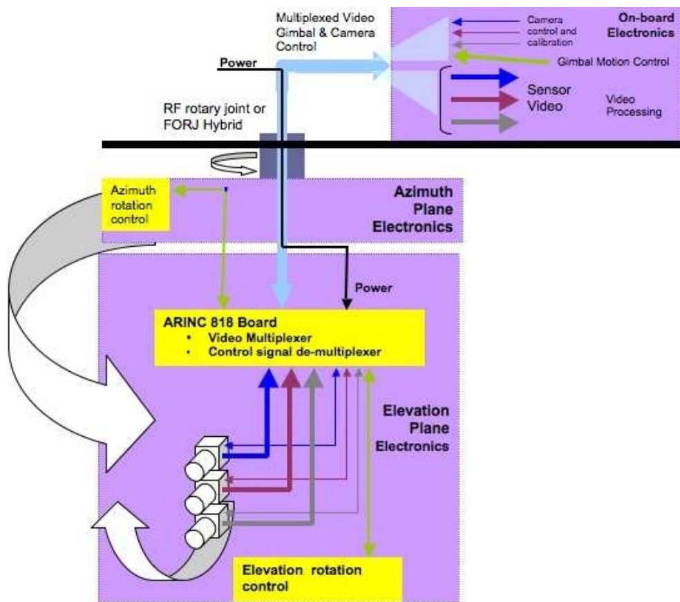
Figure 3. Example application of ARINC 818 Express.
