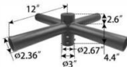
90° Quad Straight Arms
