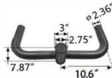
180° H-type Double Round Bullhorn Item Number : LPL-D180-HRB2.5
