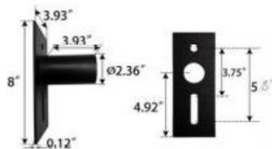
Slip Fitter Adapter Item Number : LPL-BKT-D-SFAT2.
