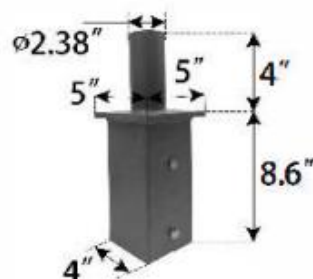
Square Tenon Adapter 5 Inch Item Number : LPL-BKT-D-RTA5
