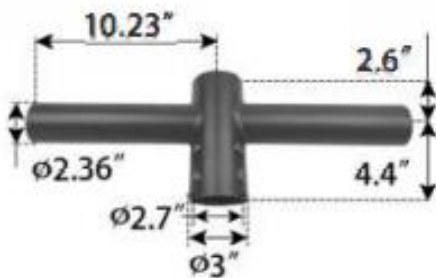
180° Double Straight Arms
