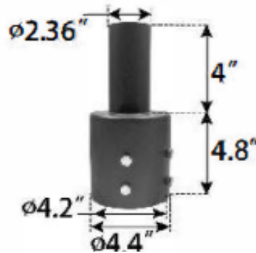
Round Tenon Adapter 4 Inch Item Number : LPL-BKT-D-RTA4
