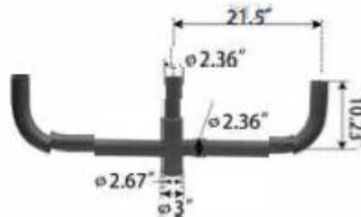
180° Triple Round Bullhorn Item Number : LPL-D180-TRB2.5
