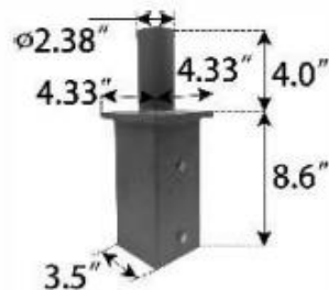
Square Tenon Adapter 4 Inch Item Number : LPL-BKT-D-STA4
