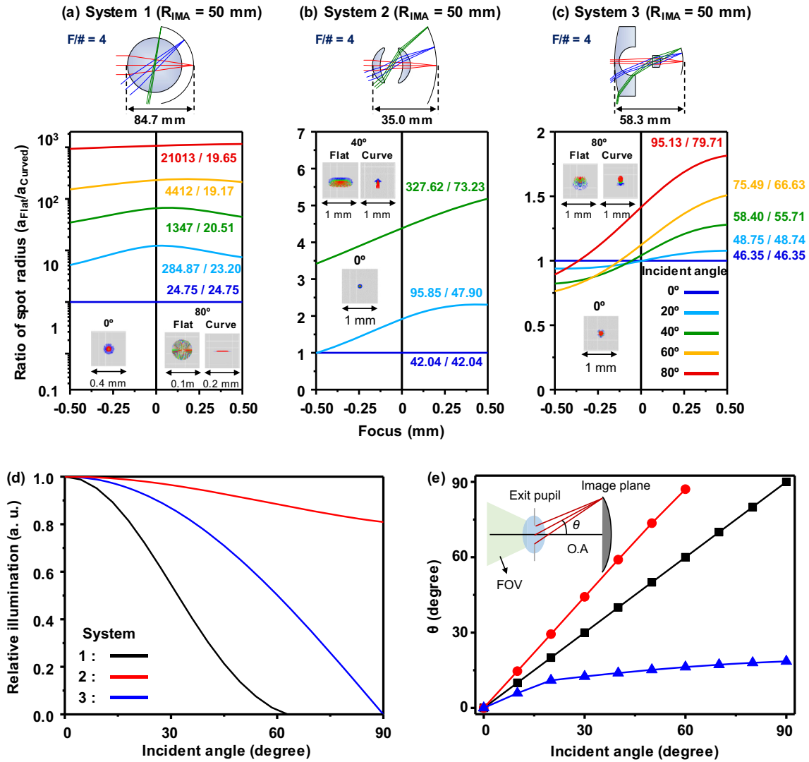
Fig. 2. Ratio of the spot radii for the flat image plane and curved image sensor ( ROC = 50 mm) with the same lens configuration, which is illustrated at the top: (a) System 1, (b) System 2, and (c) System 3. All numbers in the graphs are in \mu\text{m} and the spot sizes are at Focus = 0. The insets indicate the distribution of the light beam for wavelengths of 450, 550, and 650 nm as indicated by the blue, green, and red dots, respectively. (d) Relative illumination according to the incident angle at a wavelength of 550 nm for each system. (e) Angle \theta as a function of the incident angle at a wavelength of 550 nm for each system. The inset presents a schematic of the definition of angle \theta , which is the angle between the ray from an off-axis focal point to the center of the exit pupil and the optical axis. (For interpretation of the references to colour in this figure legend, the reader is referred to the web version of this article.)
