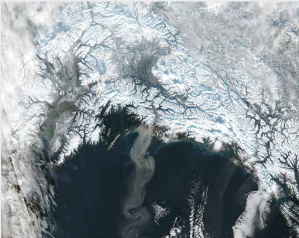
Figure 2 The Gulf of Alaska is a region of contrasts between the high mountains that surround it and the waters of the gulf. In this image from November 2017, the complex topography of the region is highlighted by the differences in snow cover between the mountaintops and the surrounding valleys. A plume of glacial dust can be seen extending from the mouth of the Copper River valley, one of the largest in the region. These plumes are the result of high winds that blow down the valley, and are an important source of nutrients for the highly productive marine ecosystem of the region.
