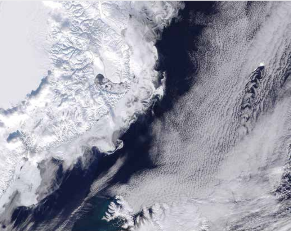
Figure 4 A winter’s view of the Denmark Strait. Complex swirls of sea ice are present along the east Greenland coast. Onshore, the mountains of the coastal region stand in juxtaposition to the smooth glaciers of the central ice cap. Offshore, a band of clouds can be seen extending south towards northern Iceland. Jan Mayen, a volcanic island that rises to a height of 2,000 metres, obstructs this flow, resulting in a striking pattern in the clouds known as a von Kármán vortex street.
