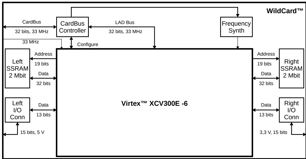
Figure 286. WildCard block diagram
