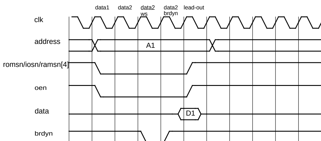
Figure 225. Read cycle with one waitstate (configured) and one BRDYN generated waitstate (synchronous sampling).
