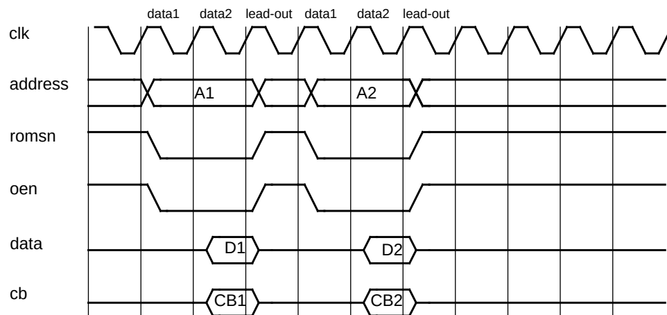
Figure 213. Prom non-consecutive read cycles.
