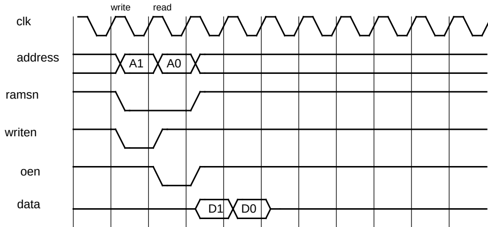
Figure 269. 32-bit SSRAM write cycle
