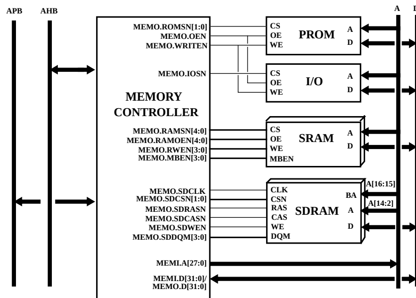
Figure 212. Memory controller connected to AMBA bus and different types of memory devices
