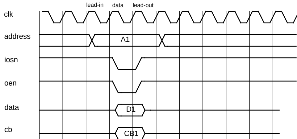
Figure 219. I/O write cycle (0-waitstates)
