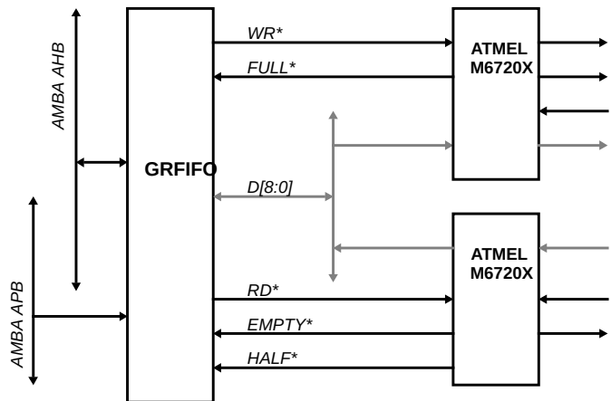
Figure 142. Example of usage, with shared external data bus
