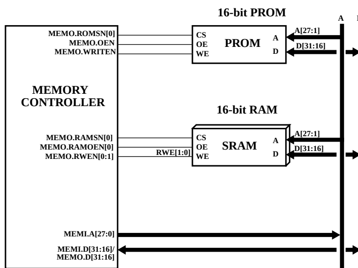
Figure 223. 16-bit memory interface example
