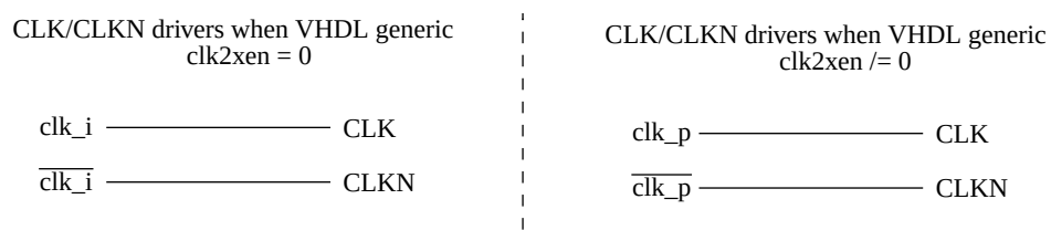
Figure 54. Spartan 3/e clock generator outputs CLK and CLKN
