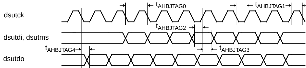
Figure 9. Timing waveforms
