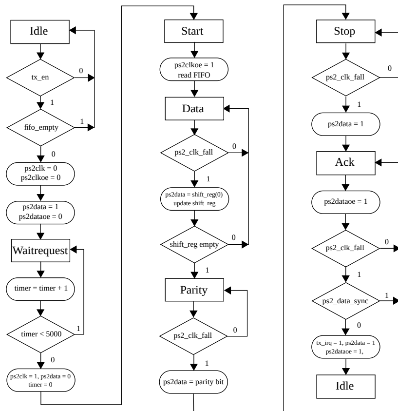
Figure 22. Flow chart for the transmitter state machine
