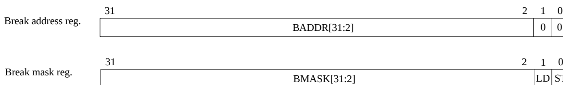
Figure 86. Trace buffer breakpoint registers
