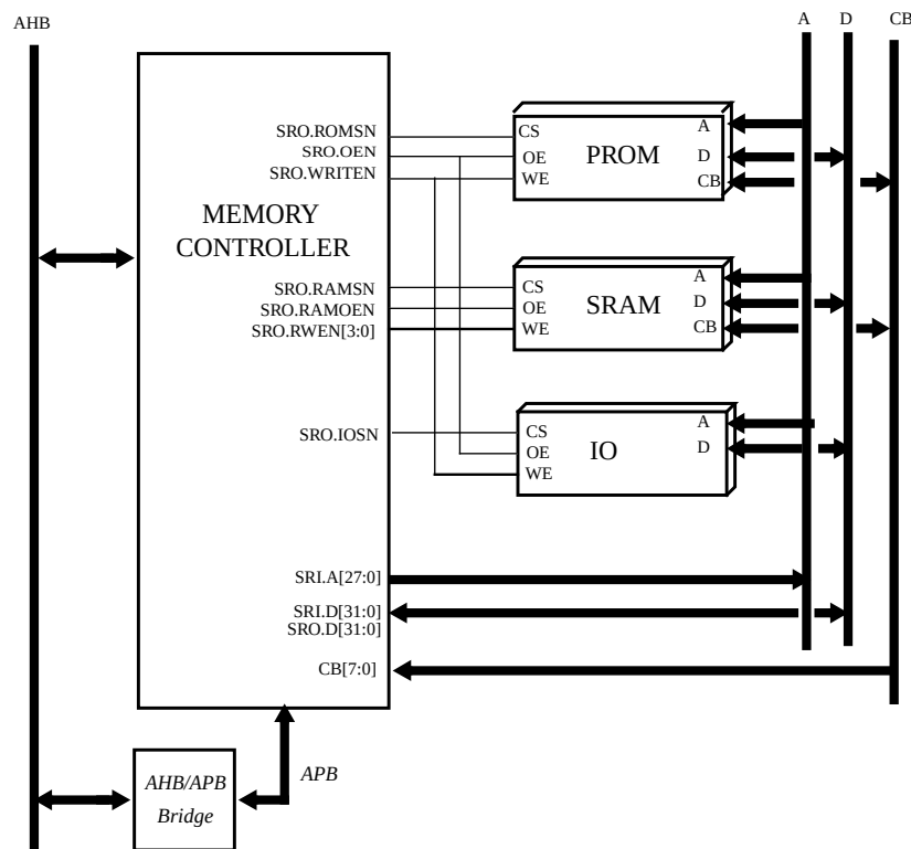
Figure 111. 32-bit FT PROM/SRAM/IO controller
