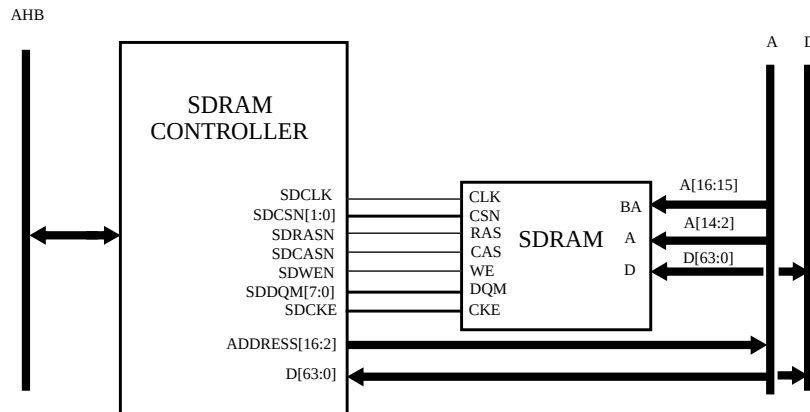
Figure 258. SDRAM Memory controller connected to AMBA bus and SDRAM
