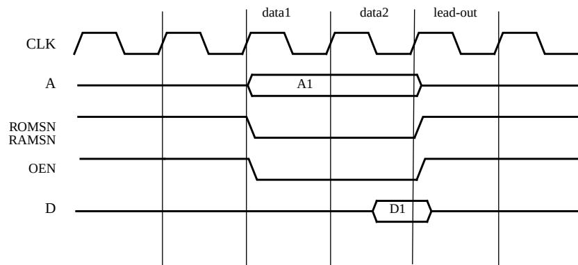
Figure 265. 32-bit PROM/SRAM/IO read cycle
