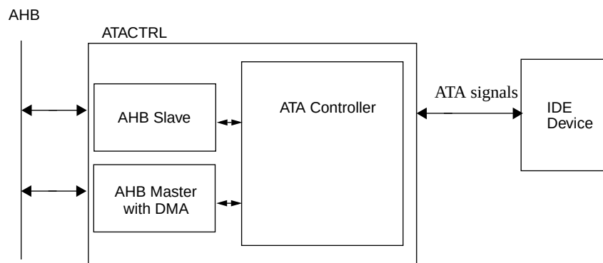
Figure 33. Block diagram of the internal structure of the ATACTRL.
