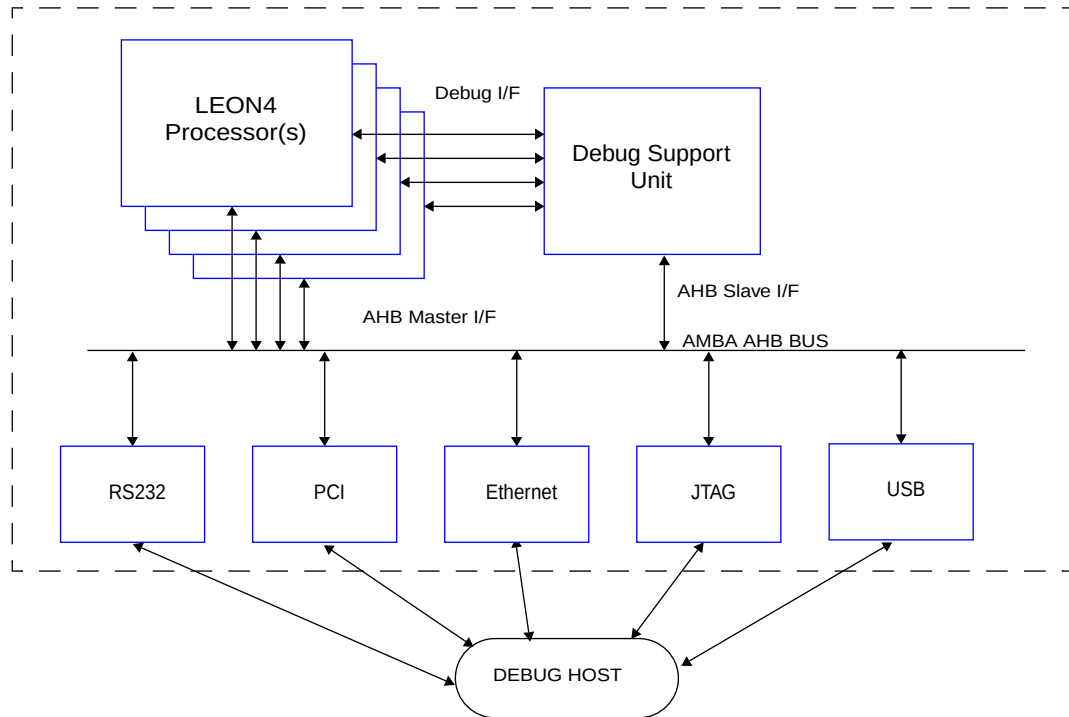
Figure 88. LEON4/DSU Connection
