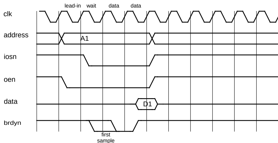
Figure 114. I/O READ cycle, programmed with 1 wait state, and with an extra data cycle added with BRDYN.
