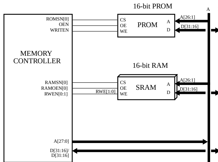
Figure 101. 16-bit memory interface example
