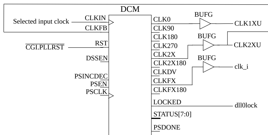
Figure 51. Spartan 3/e generation of main clock
