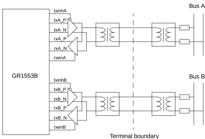
Figure 132. Interface between core and MIL-STD-1553B bus (dual-redundant, transformer coupled)
