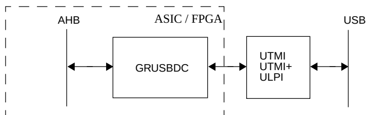
Figure 163. GRUSBDC connected to an external PHY device.
