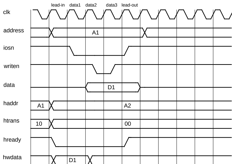
Figure 122. I/O write access with 0 wait-states.
