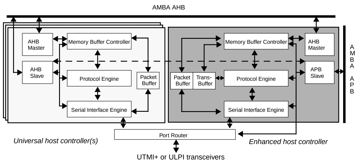
Figure 167. Block diagram of both host controller types
