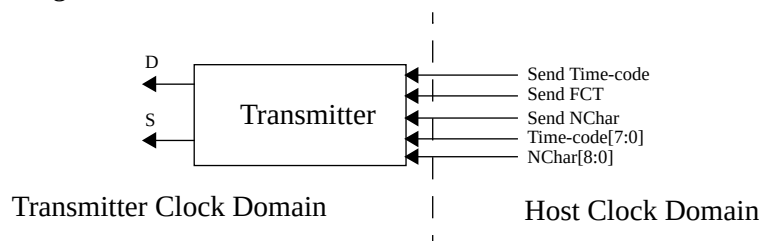
Figure 159. Schematic of the link interface transmitter.
