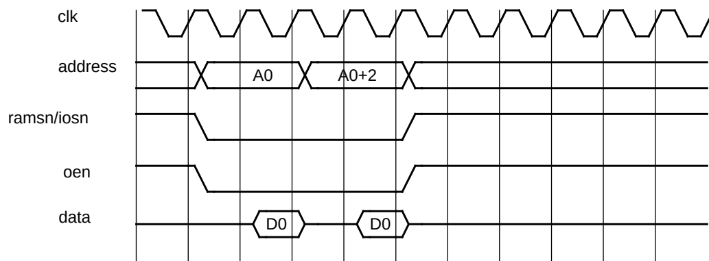
Figure 272. 32-bit PROM/IO read cycle in 16-bit mode
