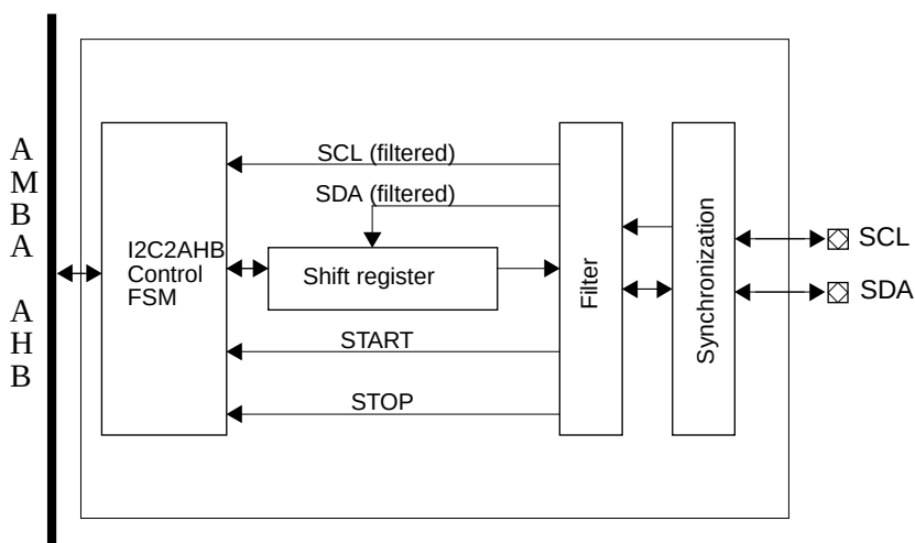
Figure 168. Block diagram, optional APB interface not shown
