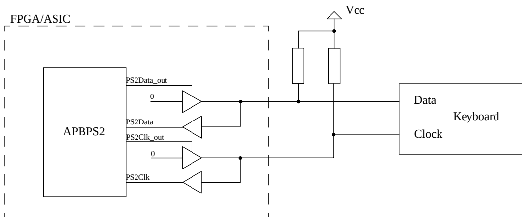
Figure 19. APBPS2 electrical interface
