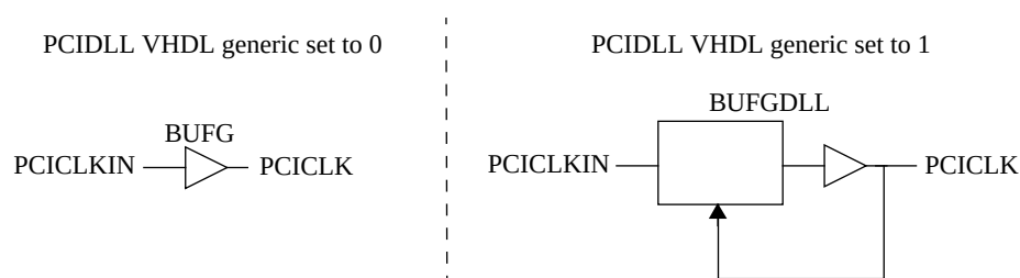
Figure 66. Virtex 2/4 PCI clock generation
