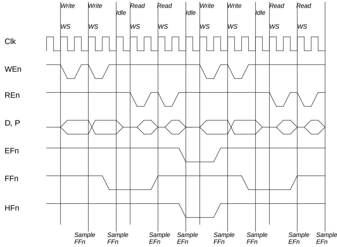
Figure 143. FIFO read and write access waveform, 0 wait states (WS)
