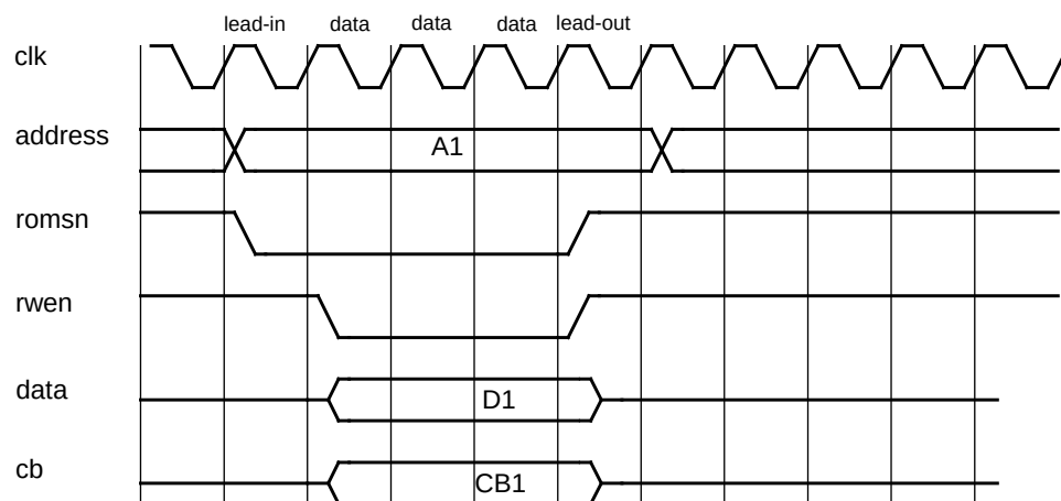
Figure 217. Prom write cycle (2-waitstates)
