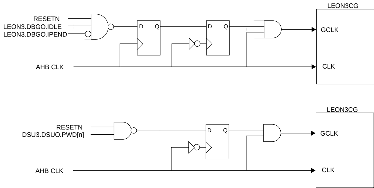
Figure 189. Examples of LEON3 clock gating
