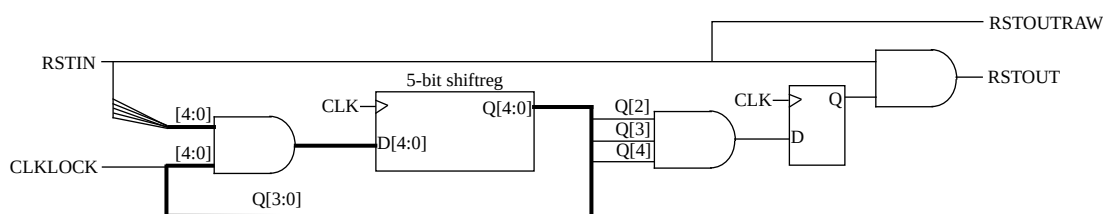
Figure 255. Reset generator with VHDL generic syncrst set to 1
