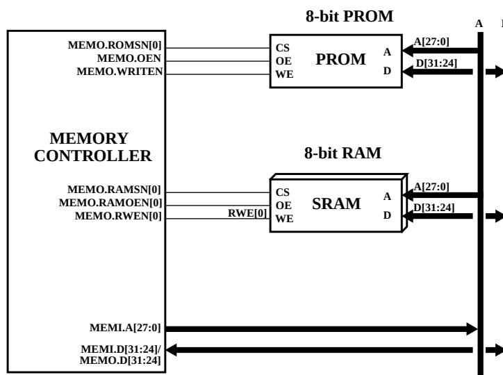
Figure 222. 8-bit memory interface example
