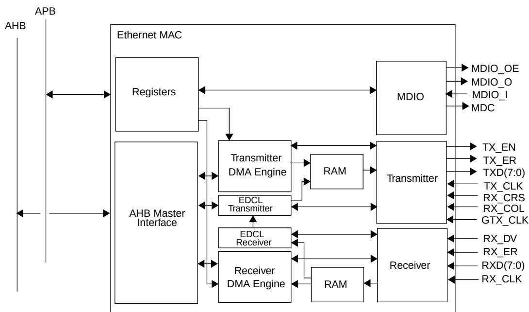
Figure 140. Block diagram of the internal structure of the GRETH_GBIT.
