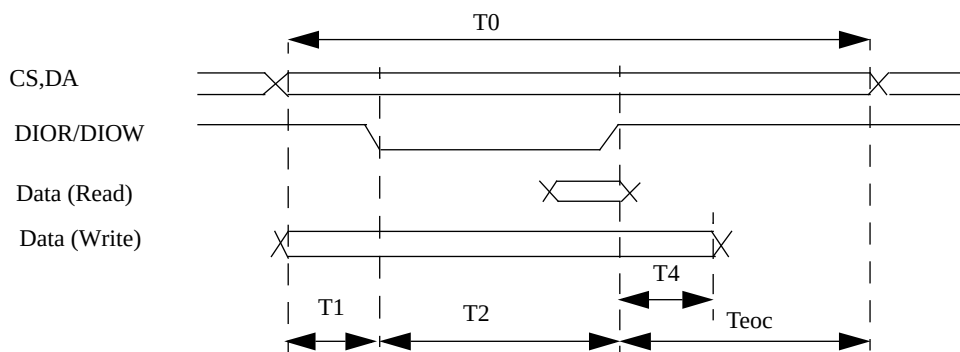
Figure 34. PIO timing diagram.
