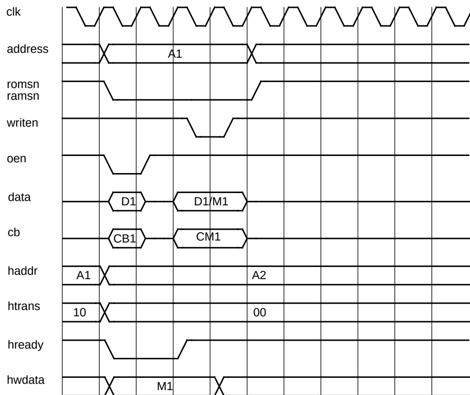
Figure 121. 32-bit PROM/SRAM rmw access with 0 wait-states and EDAC disabled.
