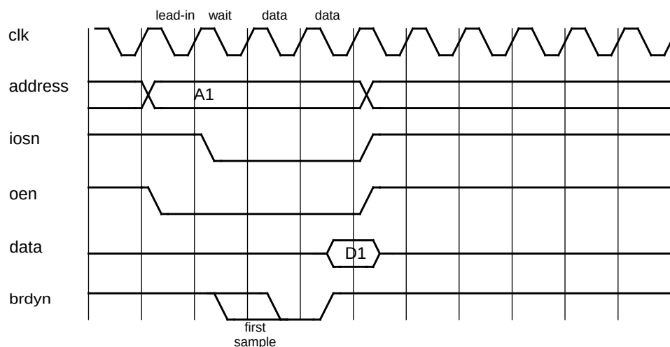
Figure 125. I/O READ cycle, programmed with 1 wait state, and with an extra data cycle added with BRDYN.
