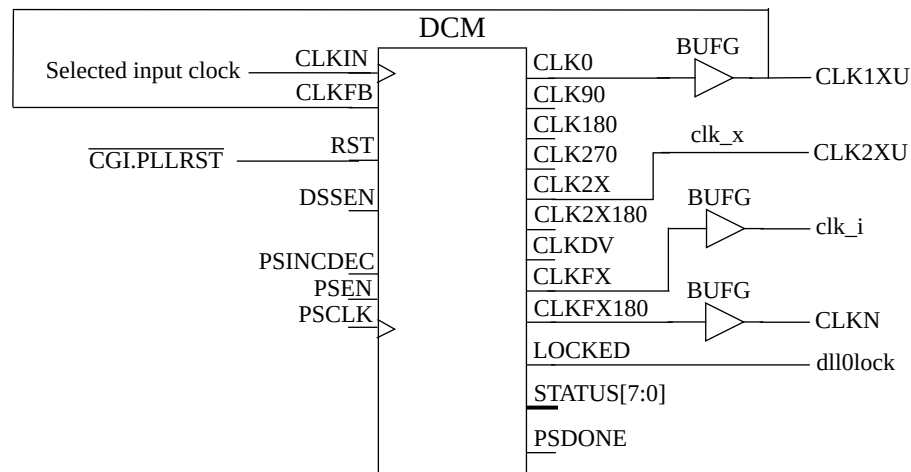
Figure 61. Virtex 2/4 generation of main clock
