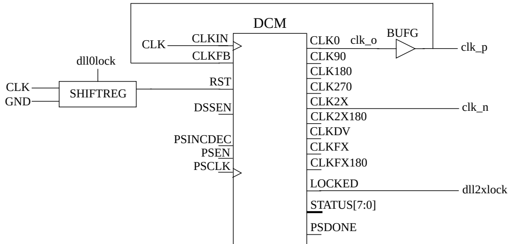
Figure 52. Spartan 3/e generation of CLK2X clock when VHDL generic clk2xen is non-zero
