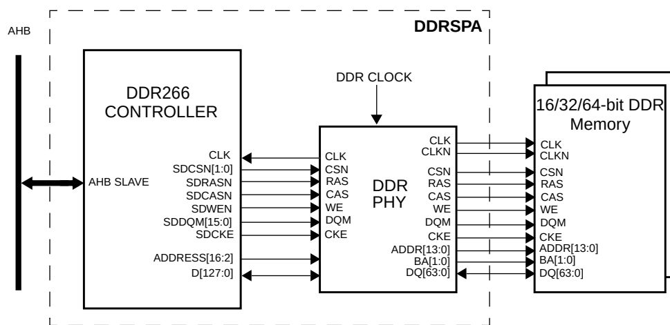
Figure 75. DDRSPA Memory controller connected to AMBA bus and DDR SDRAM
