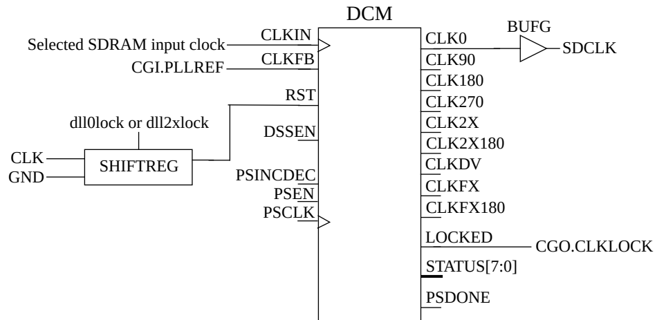
Figure 70. Virtex 5 generation of SDRAM clock
