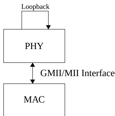
Figure 254. Block diagram of the PHY simulation model connected to a MAC.
