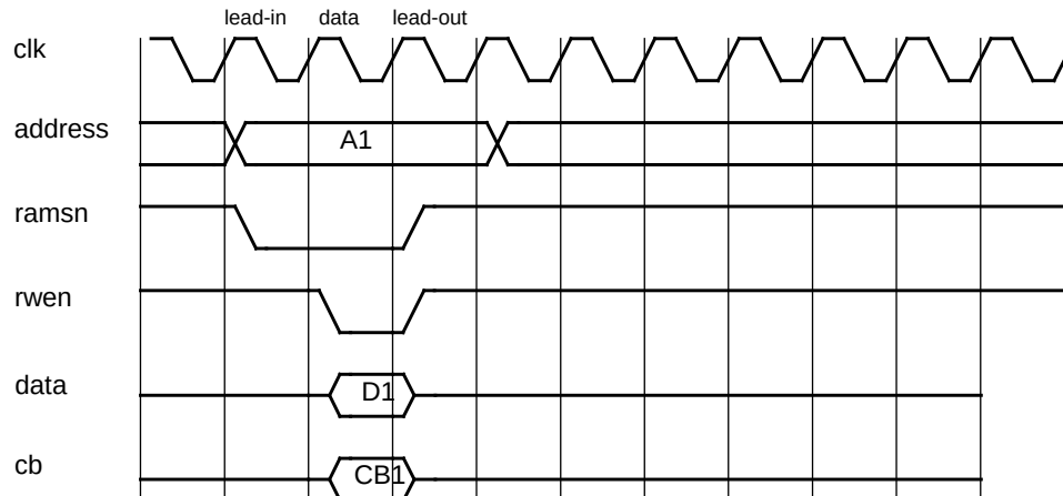
Figure 221. Sram write cycle (0-waitstates)
