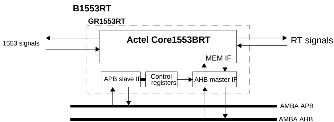
Figure 40. B1553RT block diagram
