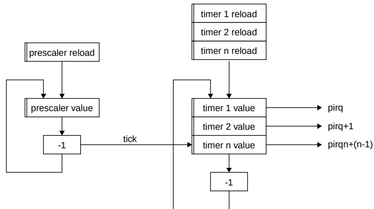
Figure 134. General Purpose Timer Unit block diagram
