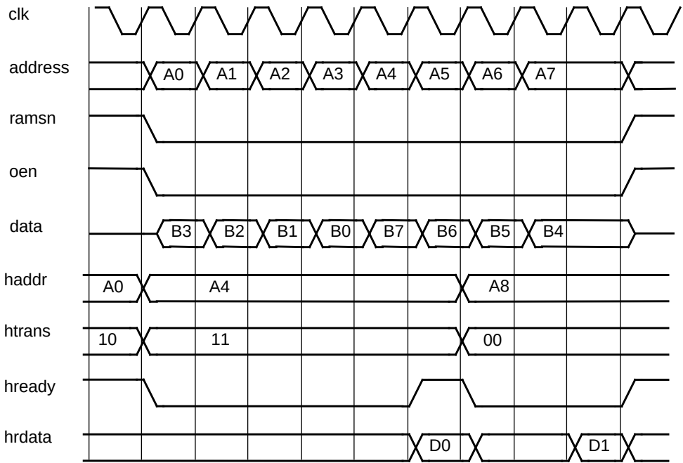
Figure 126. 32-bit SRAM sequential read accesses with 0 wait-states and EDAC enabled.
