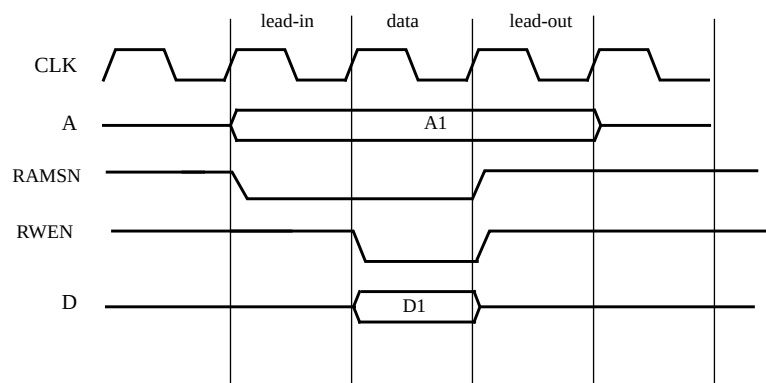
Figure 266. 32-bit PROM/SRAM/IO write cycle
