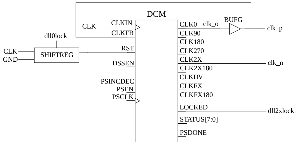
Figure 68. Virtex 5 generation of CLK2X clock when VHDL generic clk2xen is non-zero
