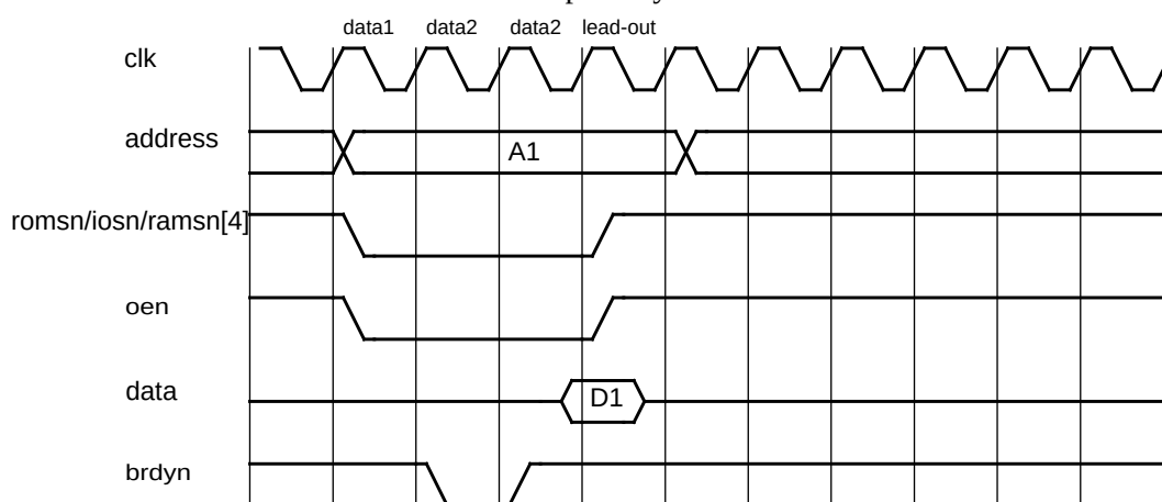
Figure 224. READ cycle with one extra data2 cycle added with BRDYN (synchronous sampling). Lead-out cycle is only applicable for I/O accesses.
