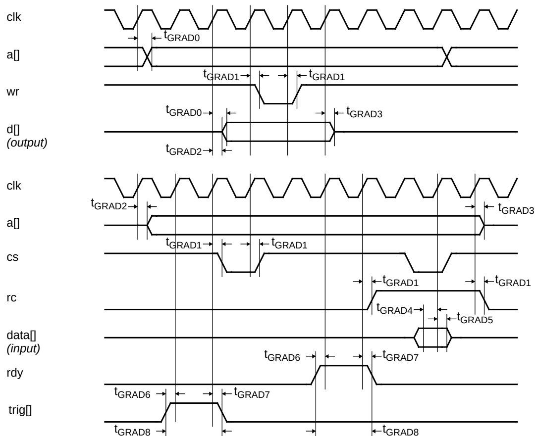
Figure 148. Timing waveforms
