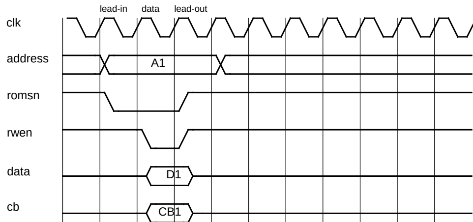
Figure 216. Prom write cycle (0-waitstates)
