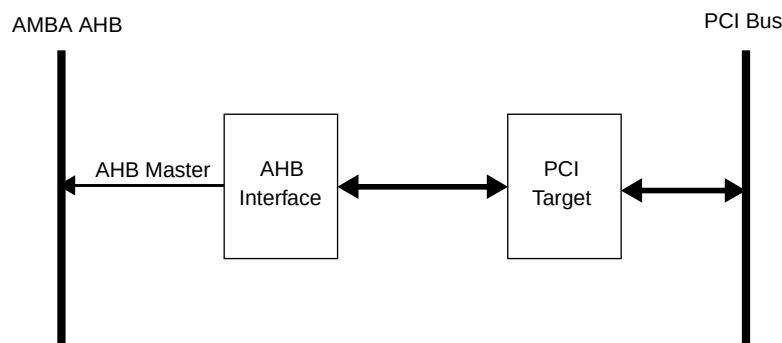
Figure 252. Target-only PCI interface
