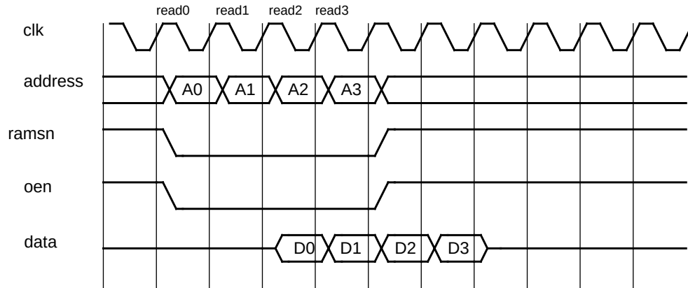
Figure 268. 32-bit SSRAM read cycle
