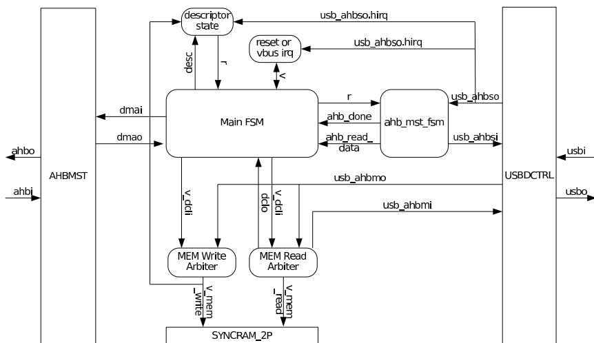
Figure 280. Block diagram of the internal structure of the GRUSBDC. Blocks with rounded corners are implemented as VHDL procedures while squares represent VHDL entities.
