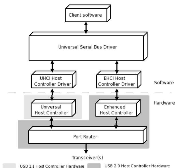
Figure 166. Block diagram of USB 2.0 host system
