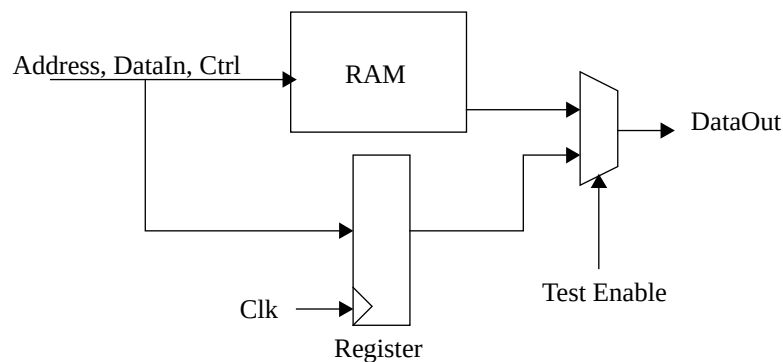
Figure 276. Scan test support
