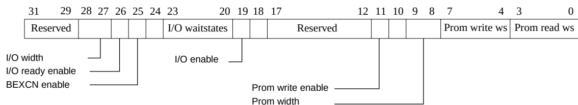
Figure 274. Memory configuration register
