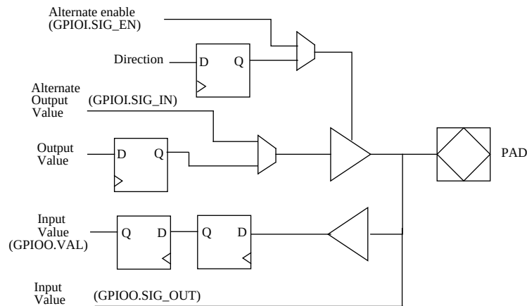
Figure 151. General Purpose I/O Port diagram
