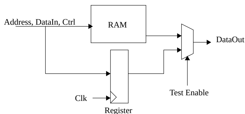
Figure 275. Scan test support
