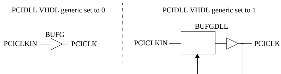
Figure 60. Virtex PCI clock generation
