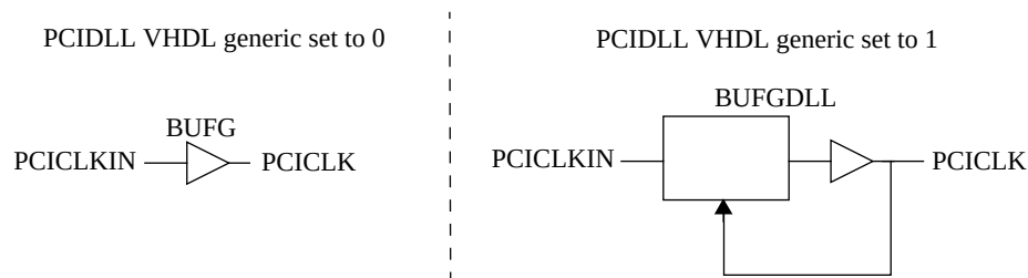
Figure 57. Spartan 3/e PCI clock generation
