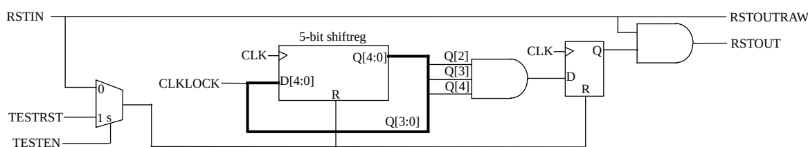
Figure 257. Reset generator with VHDL generic syncrst set to 0 and scan test enabled
