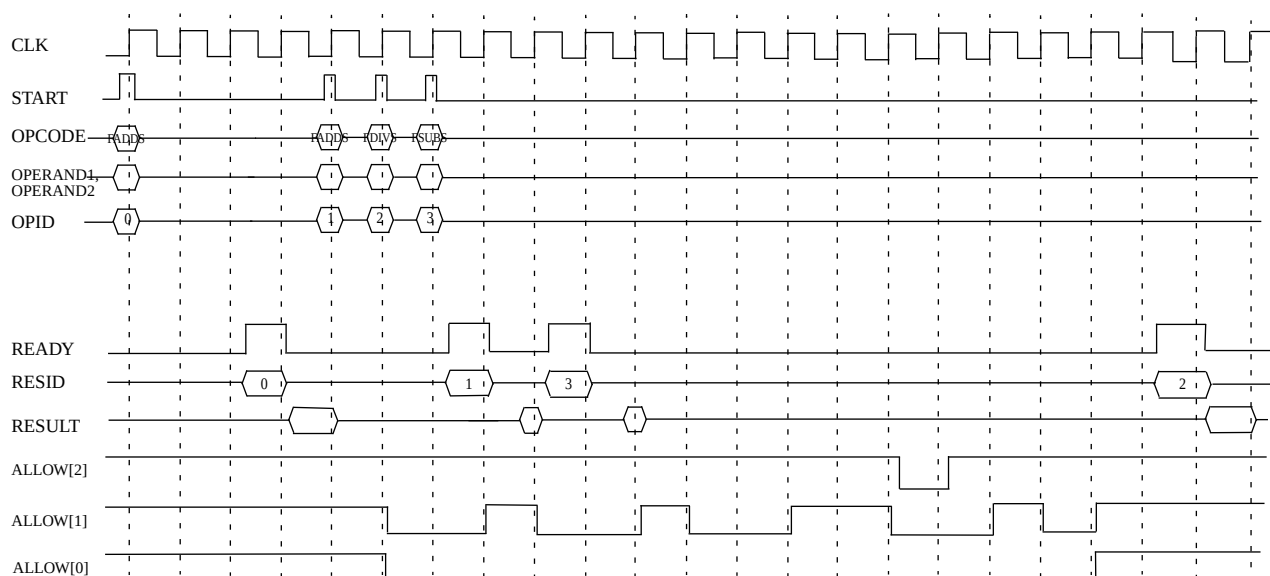
Figure 150. Signal timing
