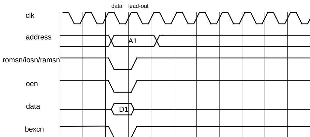
Figure 112. Read cycle with BEXCN.
