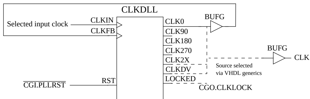
Figure 58. Virtex generation of main clock
