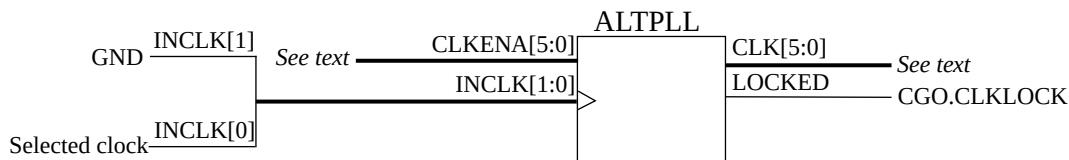
Figure 49. Altera Cyclone III ALTPLL
