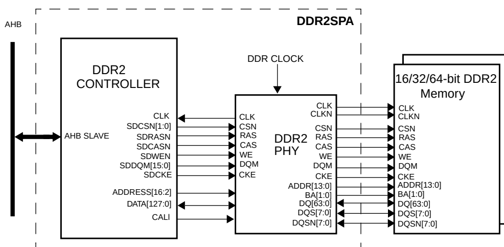
Figure 76. DDR2SPA Memory controller connected to AMBA bus and DDR2 SDRAM
