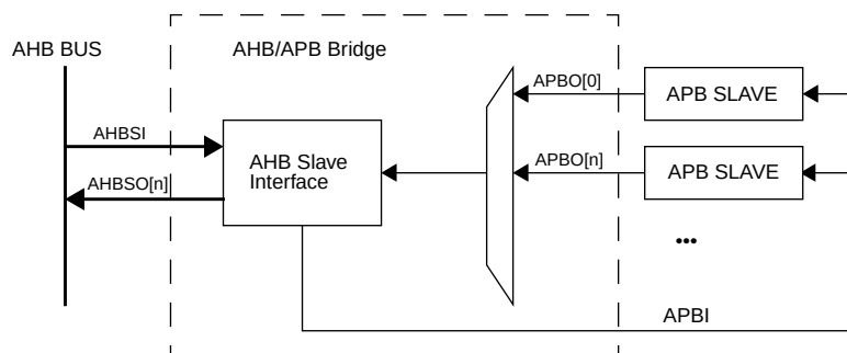
Figure 17. AHB/APB bridge block diagram
