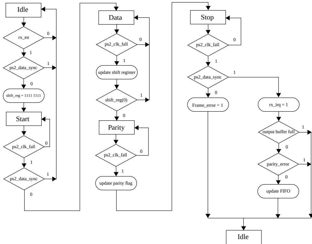
Figure 21. Flow chart for the receiver state machine
