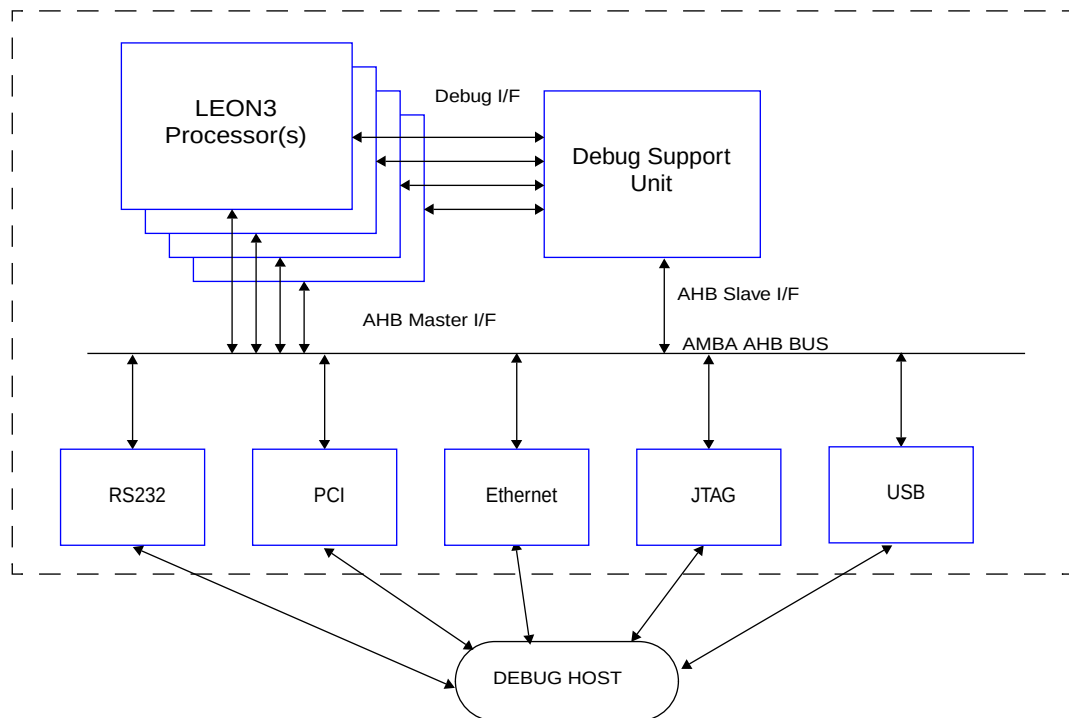
Figure 77. LEON3/DSU Connection
