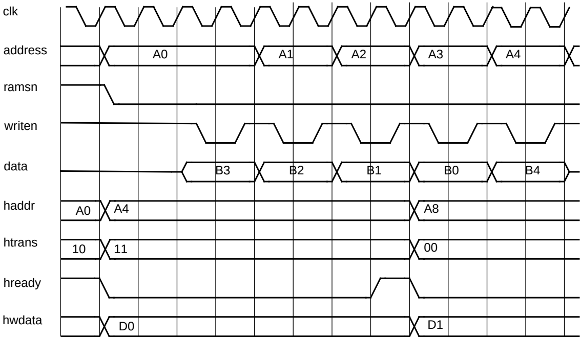
Figure 127. 32-bit SRAM sequential writeaccess with 0 wait-states and EDAC enabled.
