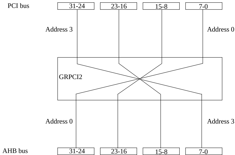
Figure 246. GRPCI2 byte twisting
