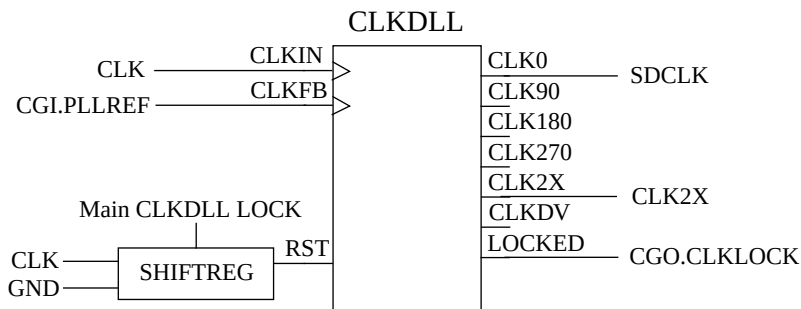
Figure 59. Virtex generation of SDRAM clock with feedback clock enabled
