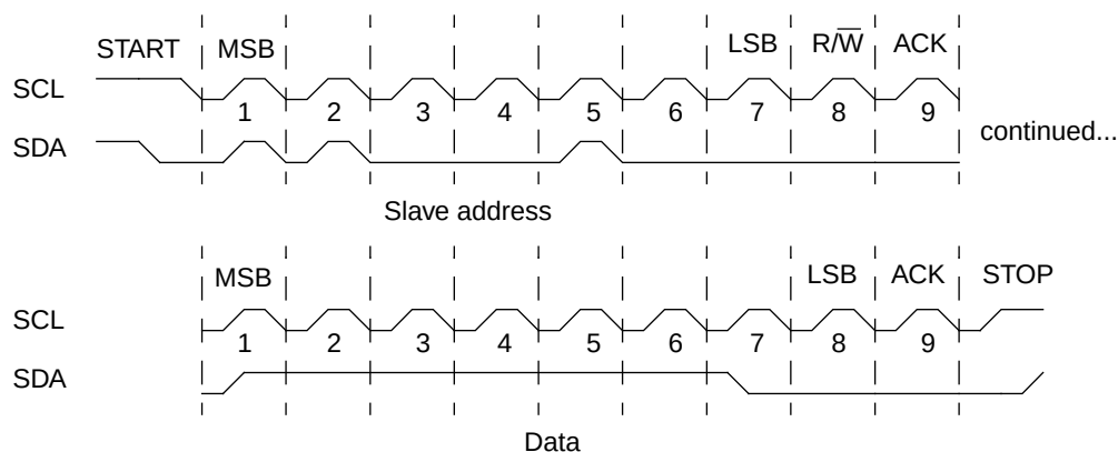
Figure 169. Complete I 2 C data transfer
