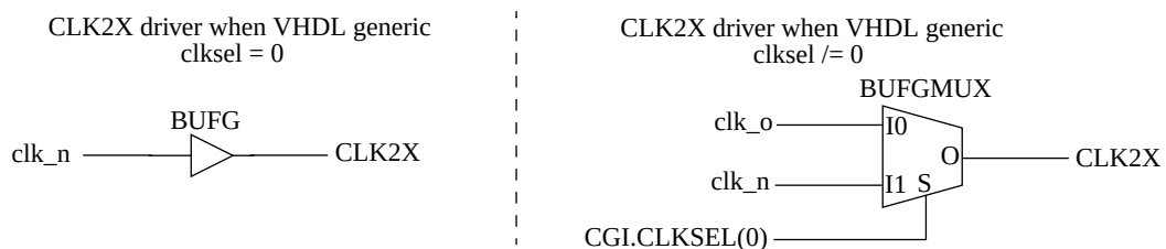
Figure 53. Spartan 3/e selection of CLK2X clock when VHDL generic clk2xen is non-zero
