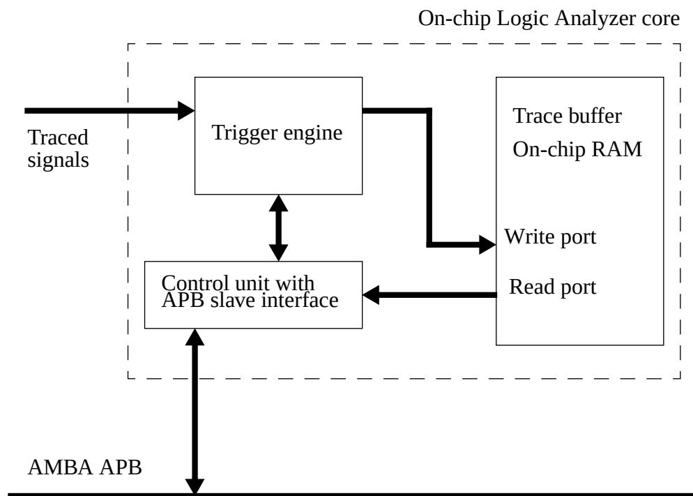
Figure 204. On-chip Logic Analyzer block diagram
