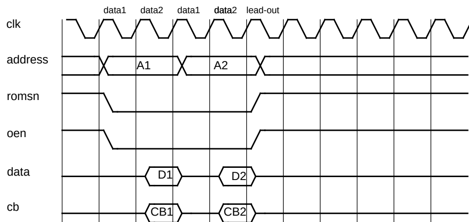
Figure 214. Prom consecutive read cycles.
