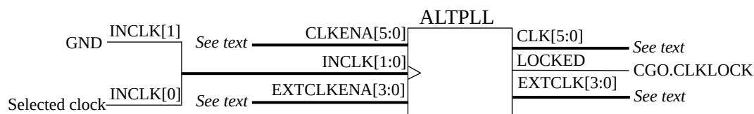
Figure 50. Altera Stratix 1/2 ALTPLL
