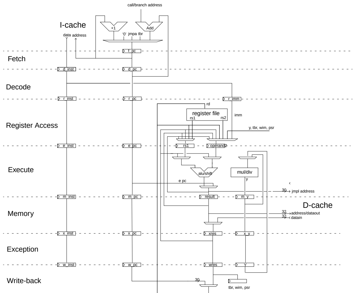
Figure 180. LEON3 integer unit datapath diagram
