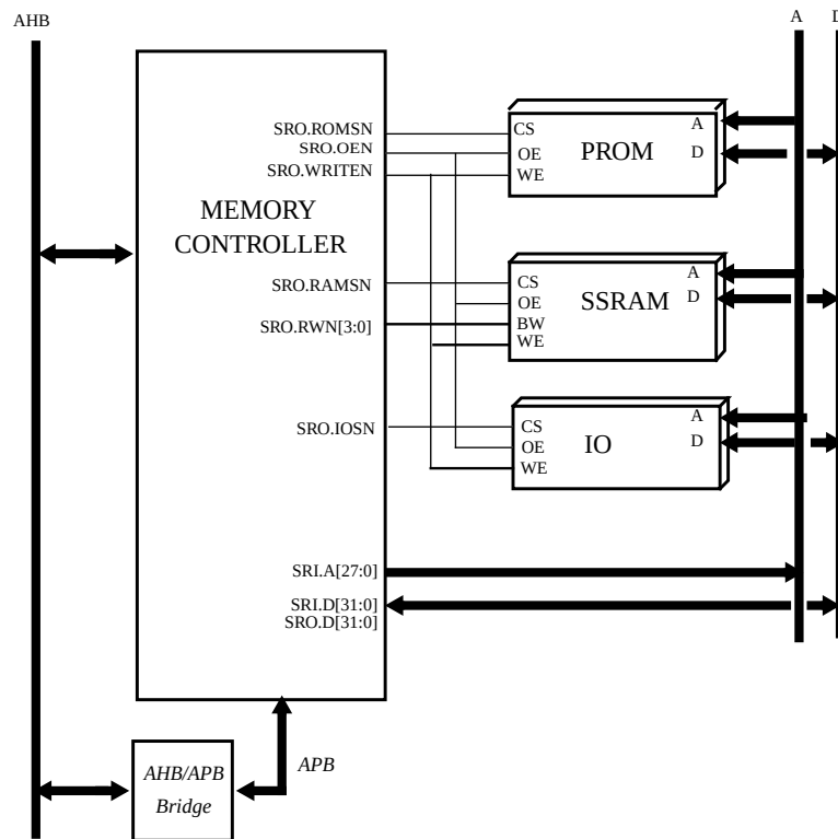
Figure 267. 32-bit SSRAM/PROM/IO controller
