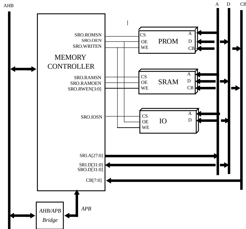
Figure 264. 8/32-bit PROM/SRAM/I/O controller
