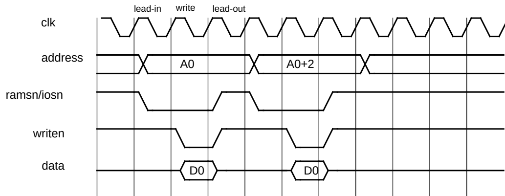
Figure 273. 32-bit PROM/IO write cycle in 16-bit mode
