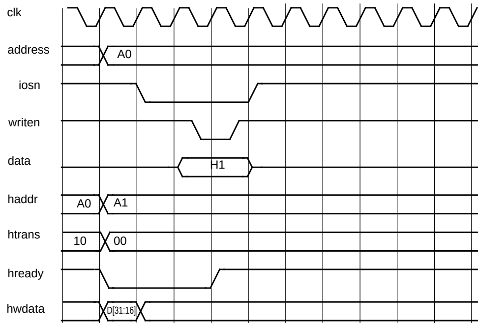
Figure 130. 16-bit I/O non-sequential write access with 0 wait-states.
