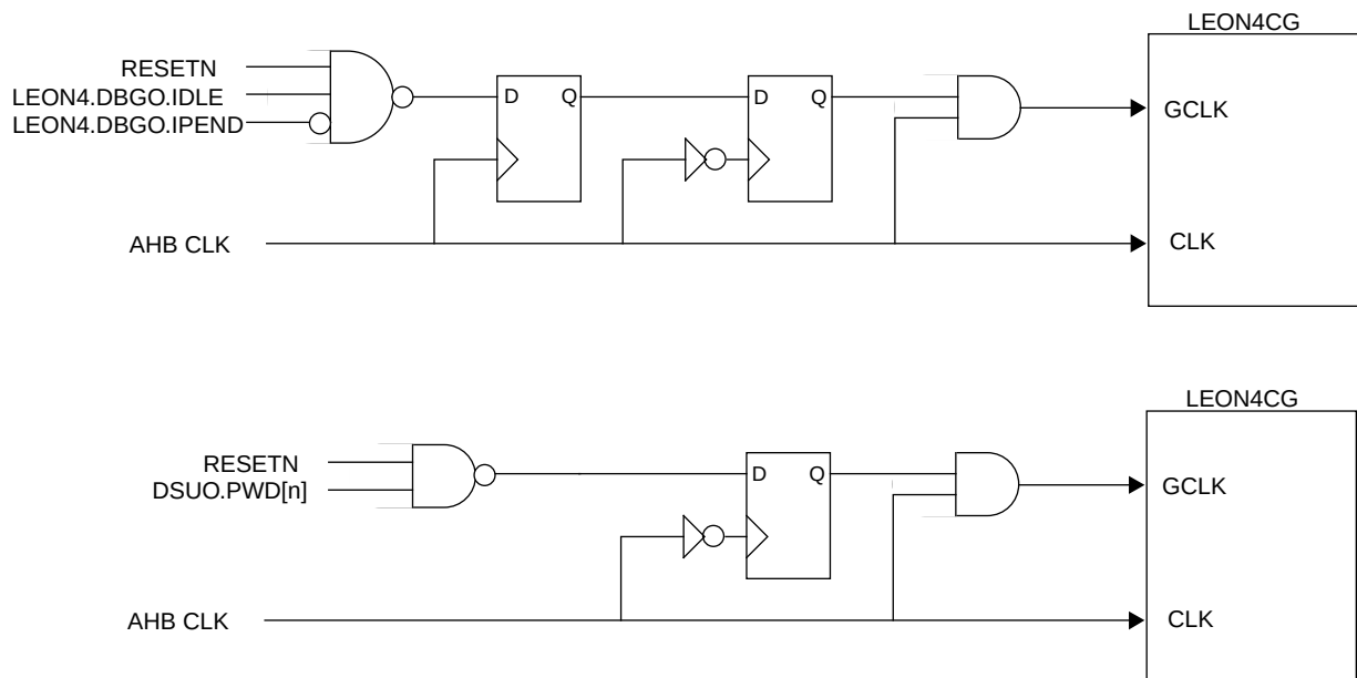
Figure 203. Examples of LEON4 clock gating
