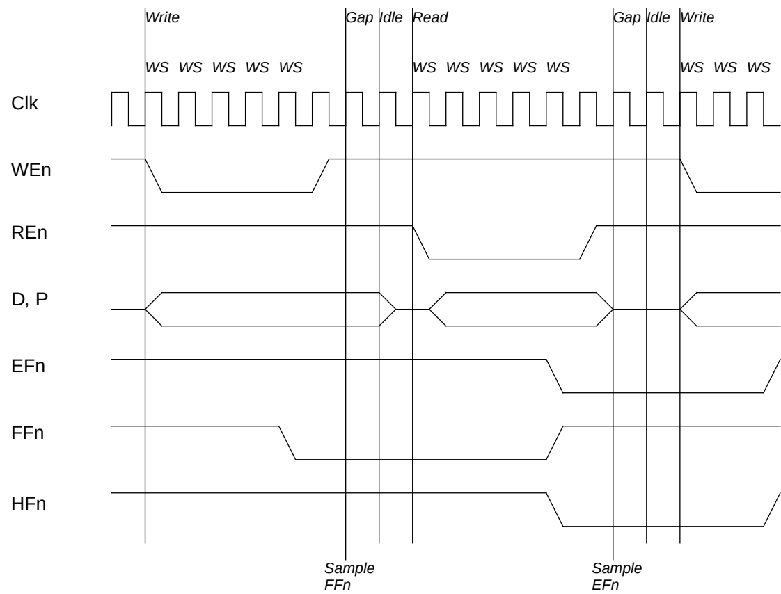
Figure 144. FIFO read and write access waveform, 4 wait states (WS)
