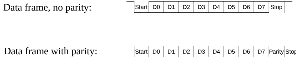
Figure 28. UART data frames
