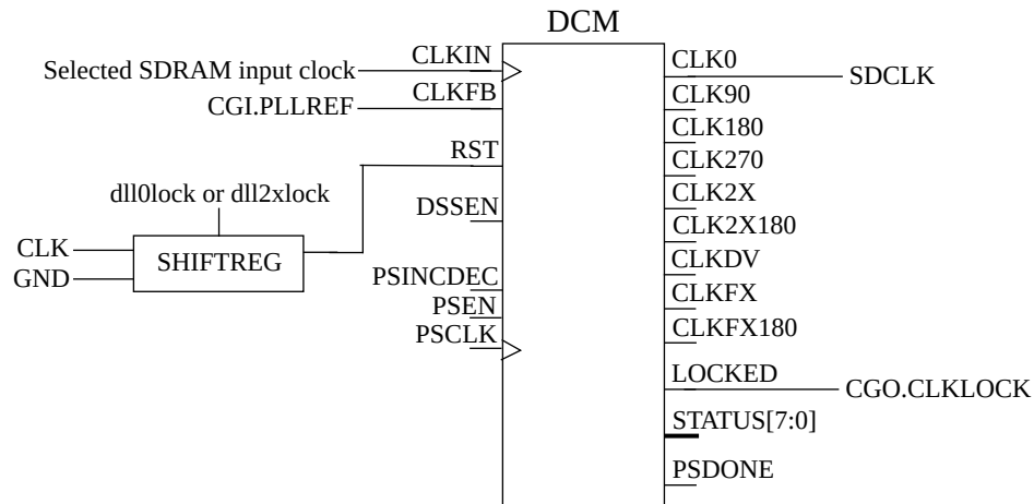
Figure 65. Virtex 2/4 generation of SDRAM clock
