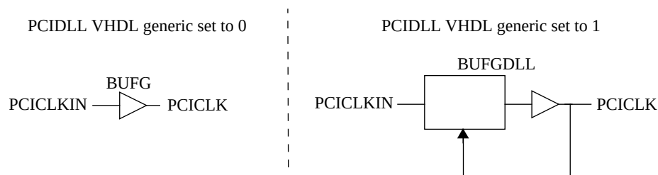
Figure 71. Virtex 5 PCI clock generation
