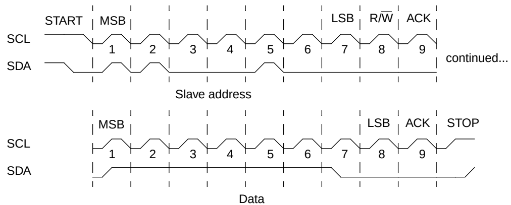
Figure 171. Complete I 2 C data transfer
