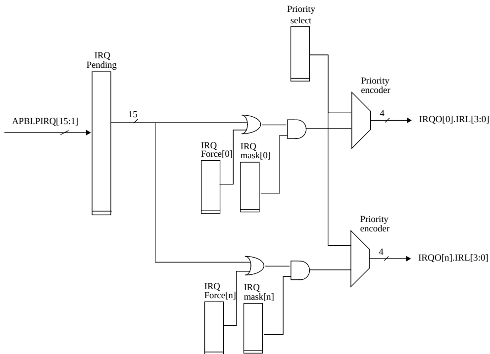
Figure 175. Interrupt controller block diagram
