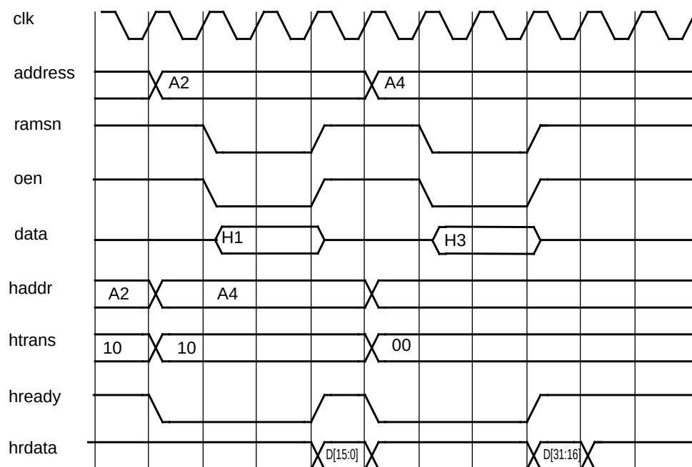
Figure 131. 16-bit I/O non-sequential read access with 0 wait-states.
