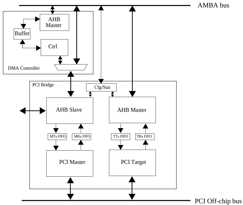
Figure 247. DMA Controller unit
