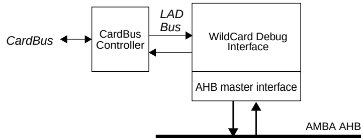
Figure 284. WildCard Debug Interface block diagram
