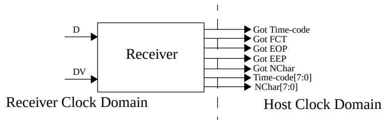
Figure 160. Schematic of the link interface receiver.
