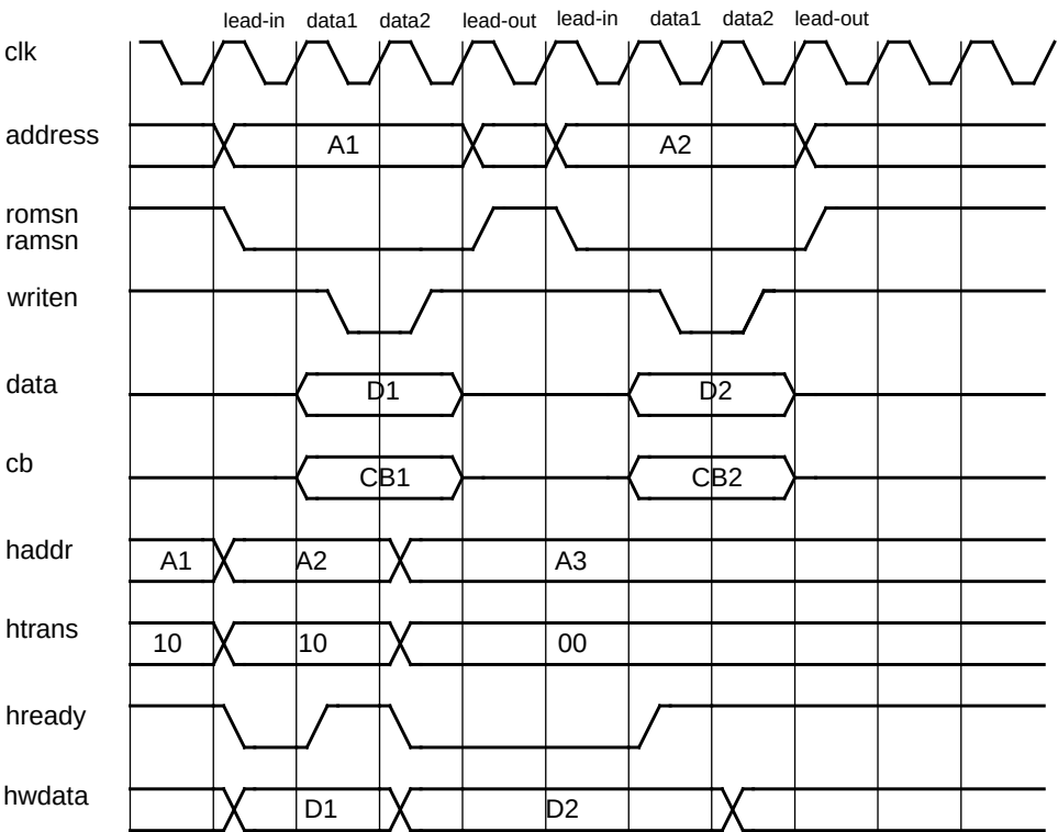
Figure 119. 32-bit PROM/SRAM non-sequential write access with 0 wait-states and EDAC disabled.
