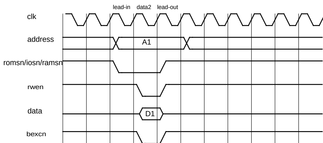
Figure 106. Write cycle with BEXCN. Chip-select (iosn) is not asserted in lead-in cycle for io-accesses.
