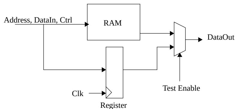
Figure 277. Scan test support
