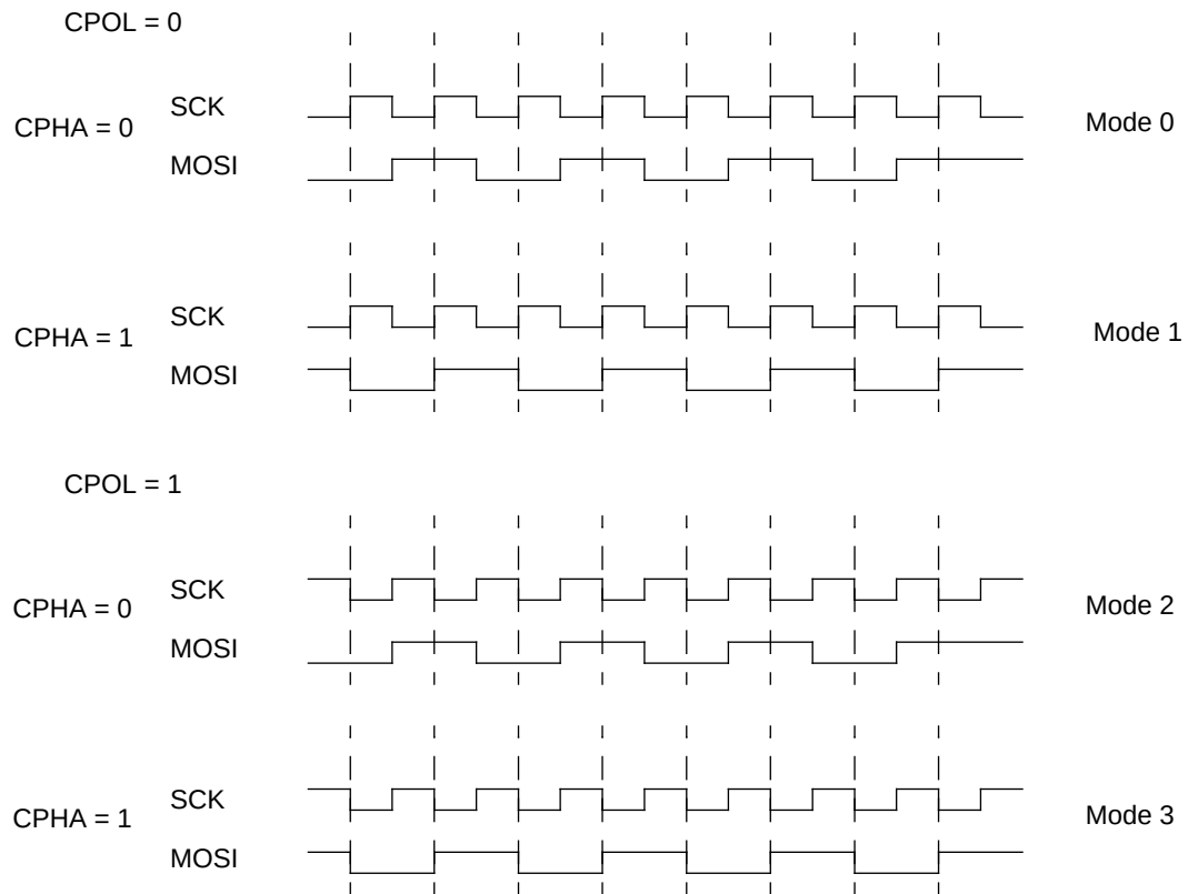
Figure 260. SPI transfer of byte 0x55 in all modes
