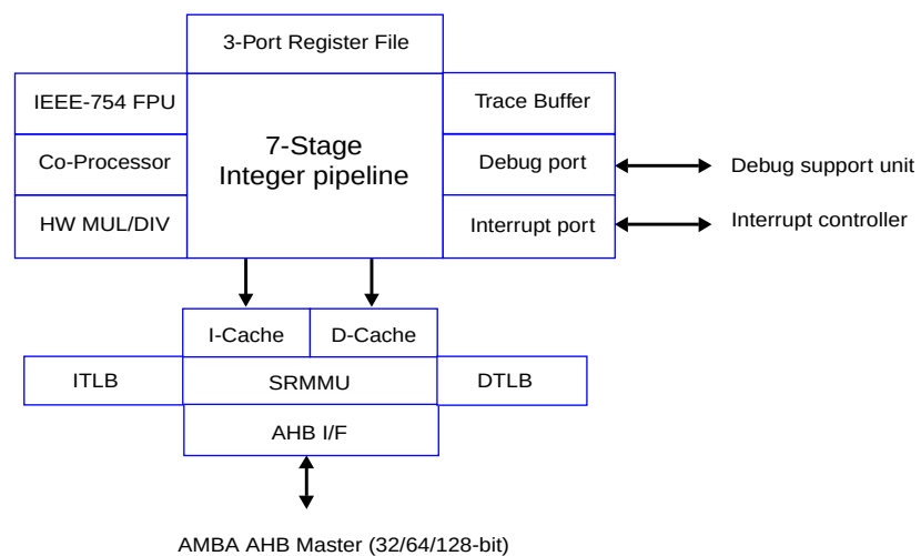
Figure 194. LEON4 processor core block diagram
