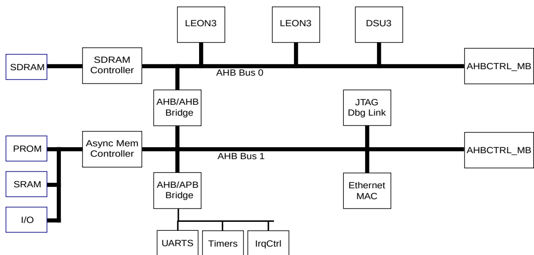
Figure 5. System with multiple AHB buses
