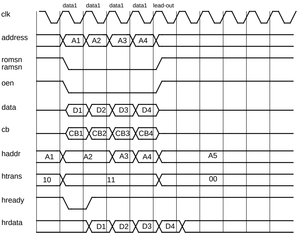
Figure 116. 32-bit PROM/SRAM sequential read access with 0 wait-states and EDAC disabled.
