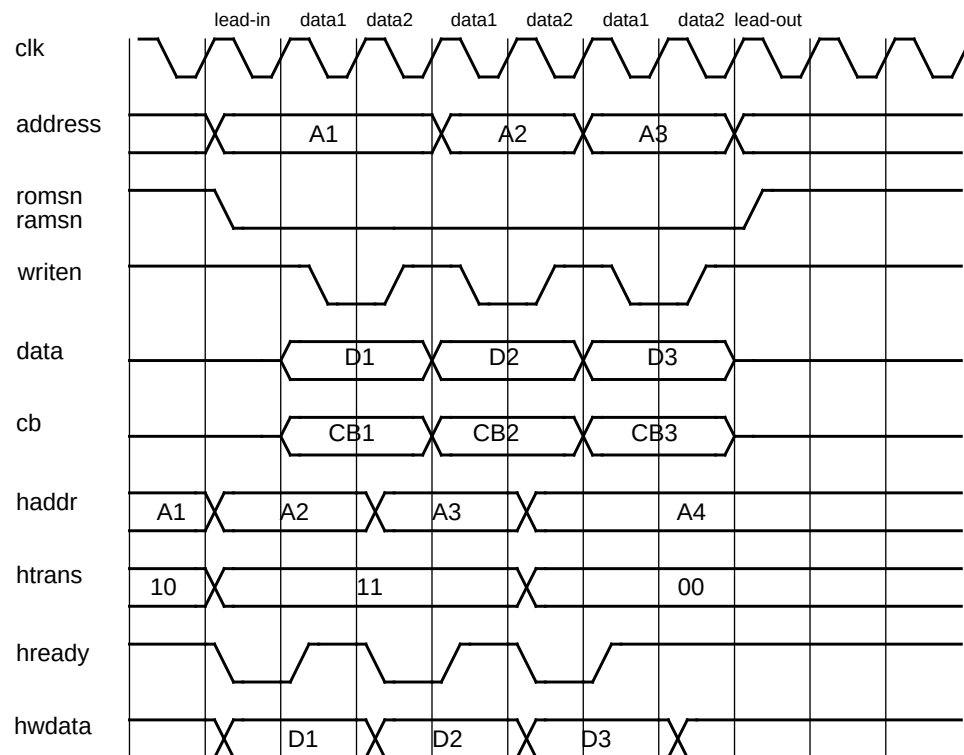
Figure 120. 32-bit PROM/SRAM sequential write access with 0 wait-states and EDAC disabled.
