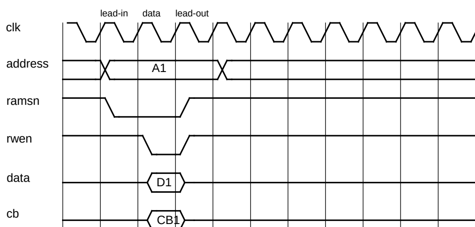
Figure 99. Sram write cycle (0-waitstates)
