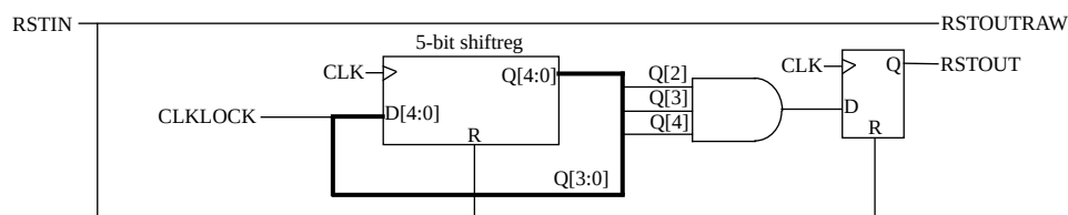
Figure 256. Reset generator with VHDL generic syncrst set to 0 and scan test disabled
