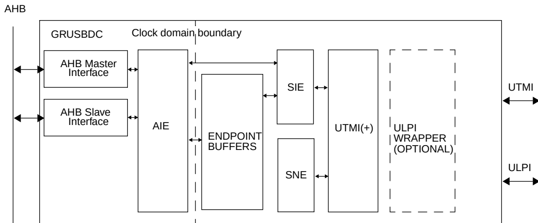
Figure 164. Block diagram of the internal structure of the core.
