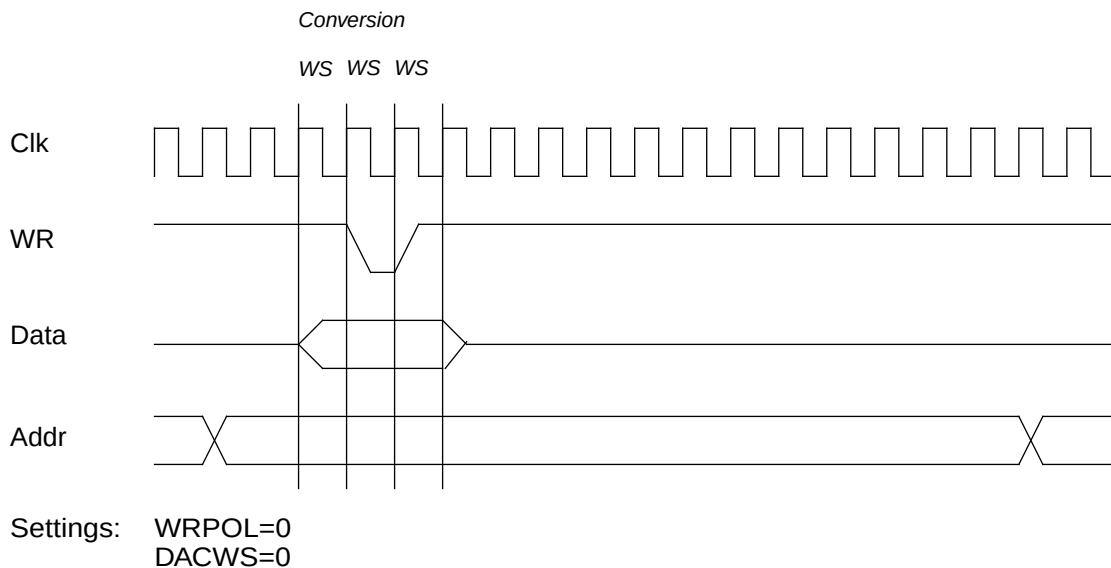
Figure 147. Digital to analogue conversion waveform, 0 wait states (WS)
