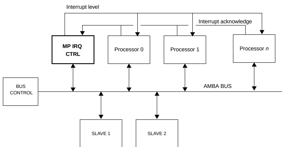
Figure 174. LEON multiprocessor system with Multiprocessor Interrupt controller
