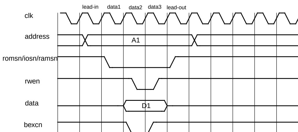
Figure 113. Write cycle with BEXCN.
