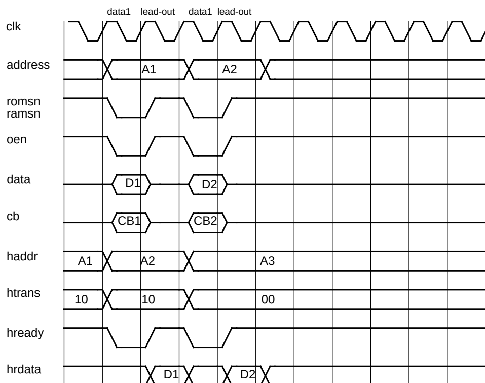
Figure 115. PROM/SRAM non-consecutive read cycles.
