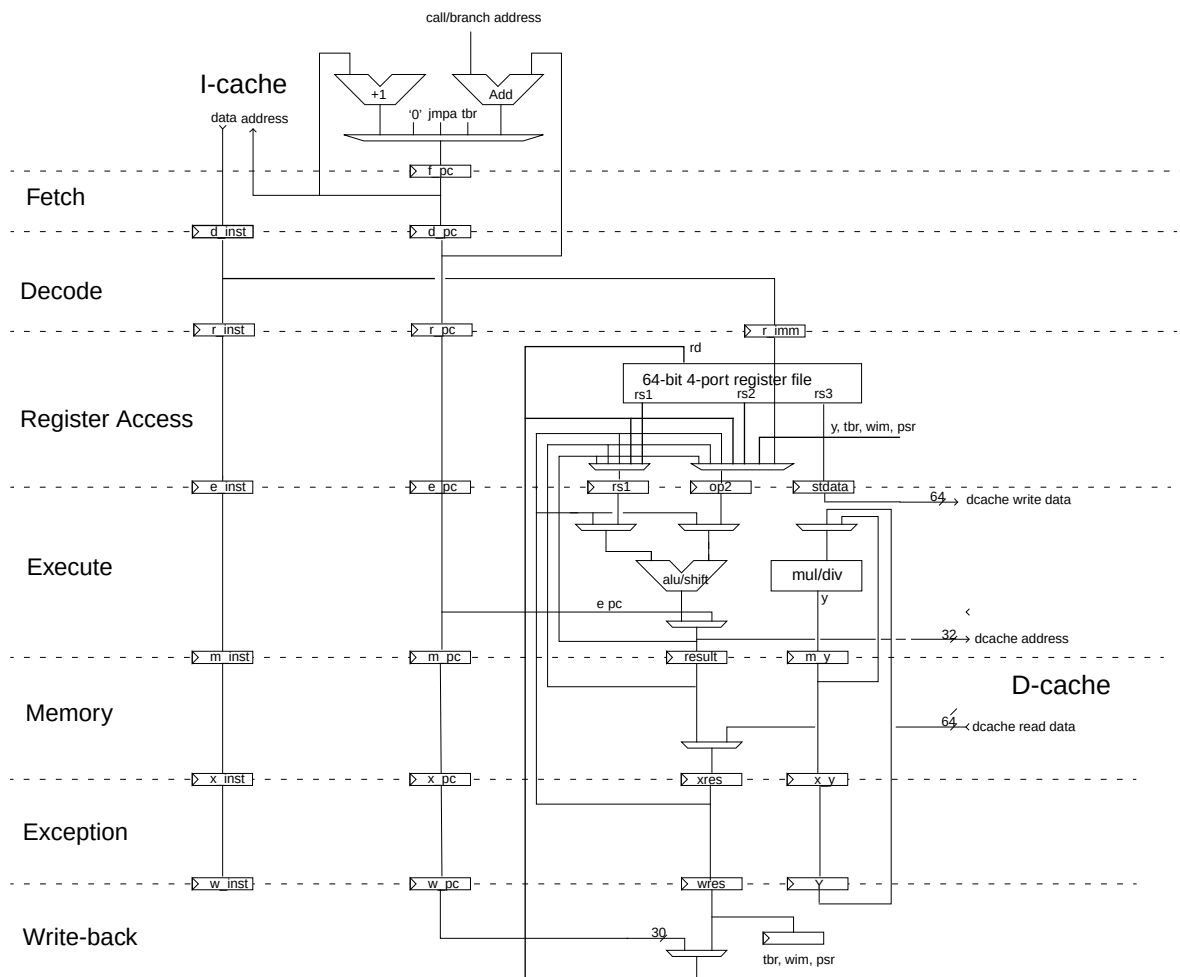
Figure 195. LEON4 integer unit datapath diagram
