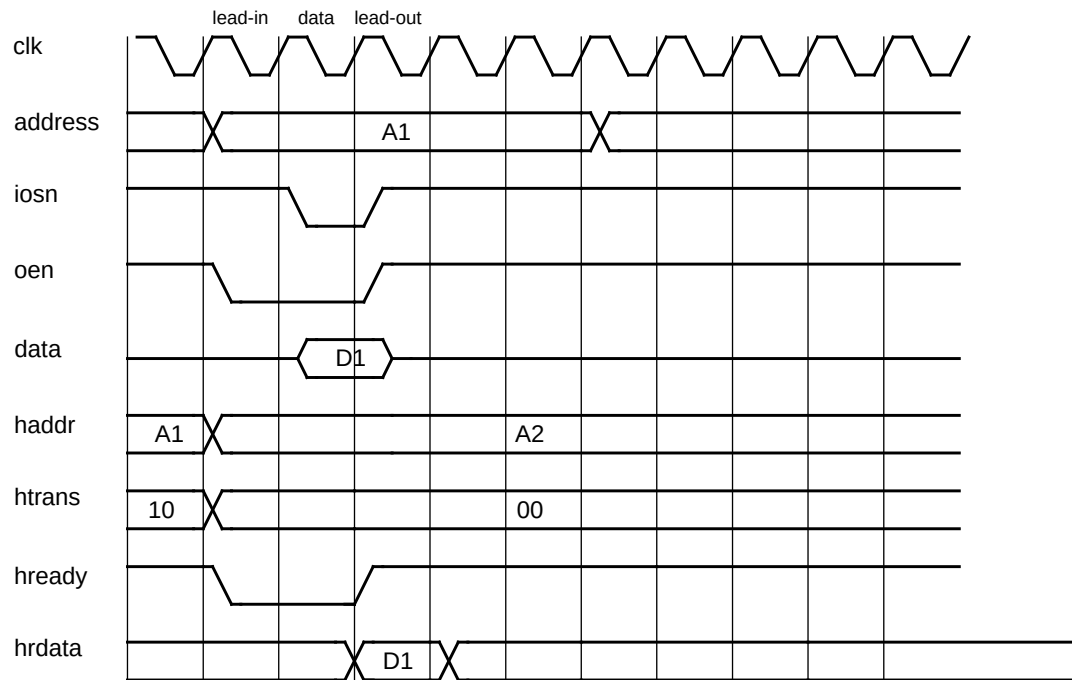
Figure 123. I/O read access with 0 wait-states
