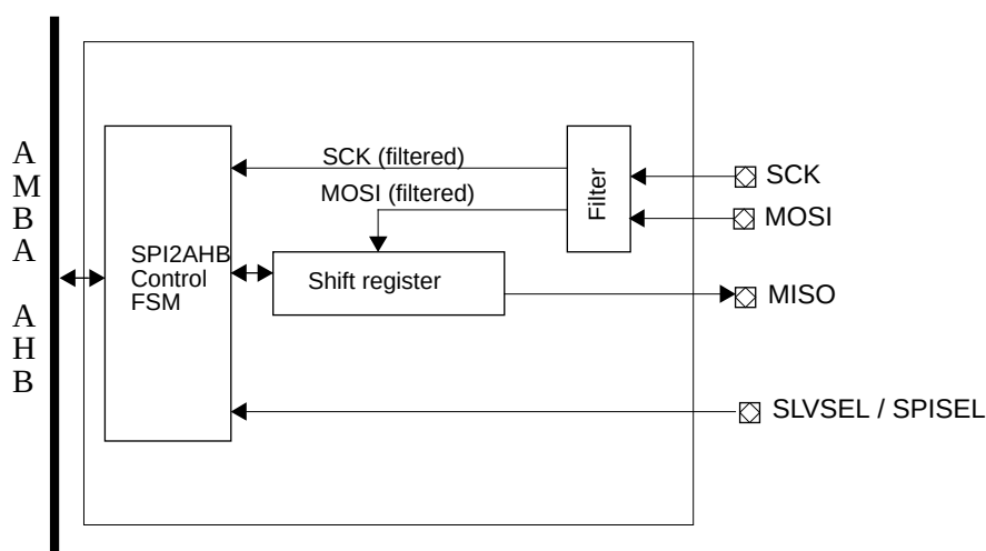
Figure 259. Block diagram, optional APB interface not shown
