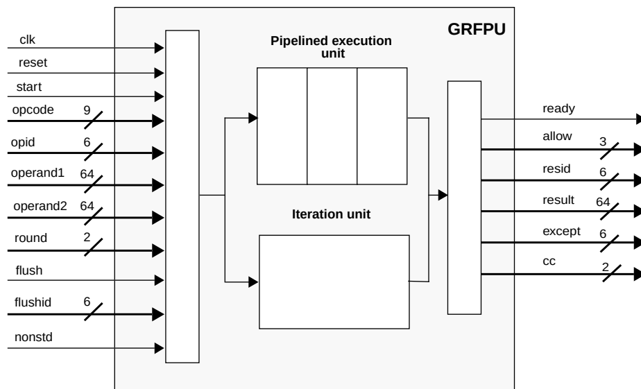
Figure 149. GRFPU Logical View
