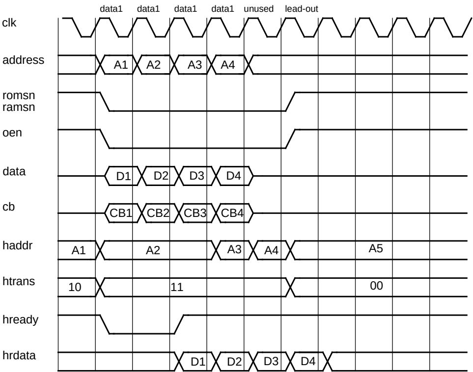
Figure 118. 32-bit PROM/SRAM sequential read access with 0 wait-states and EDAC enabled..
