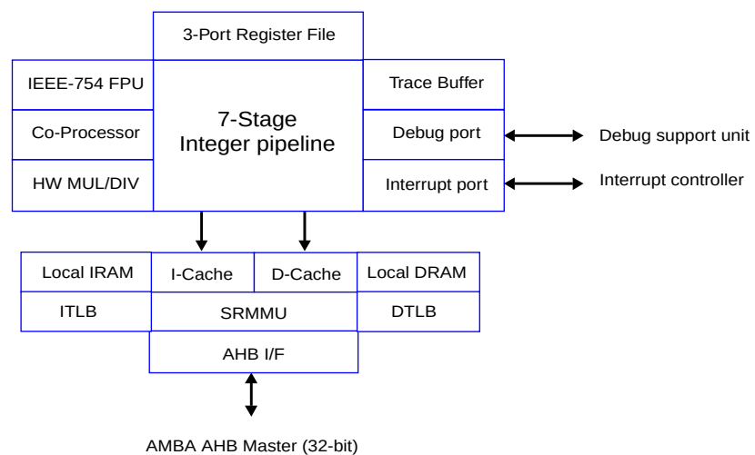
Figure 179. LEON3 processor core block diagram
