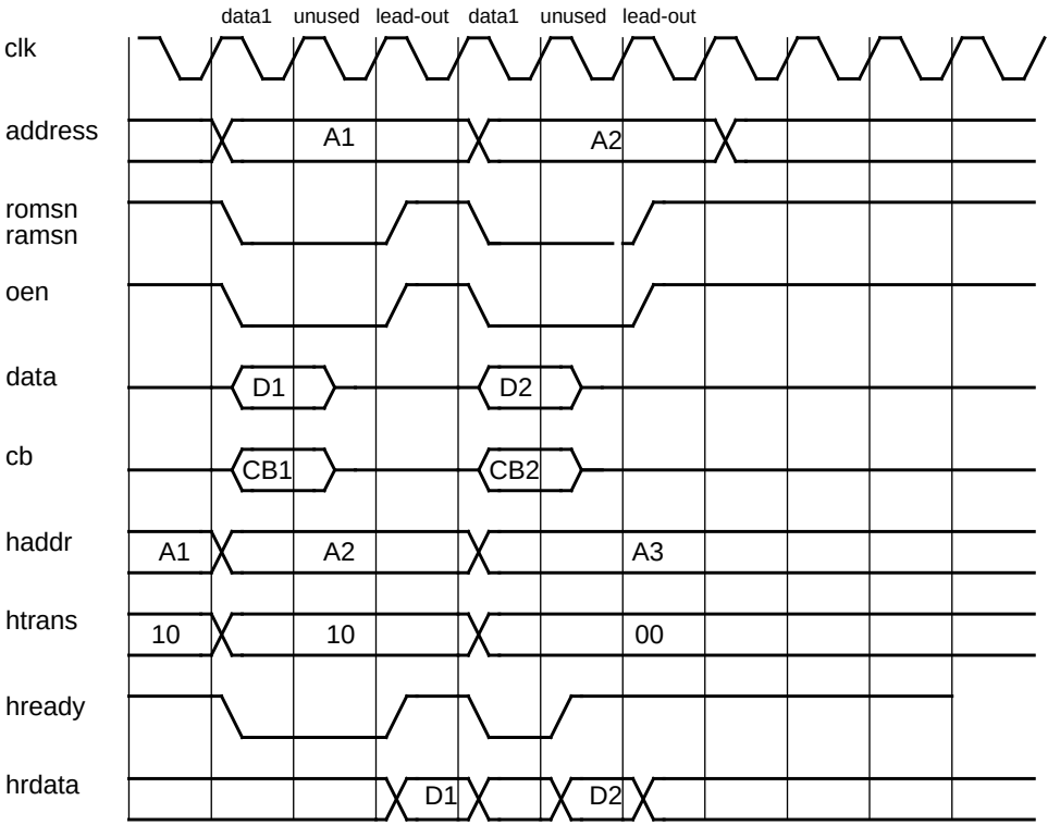
Figure 117. 32-bit PROM/SRAM non-sequential read access with 0 wait-states and EDAC enabled.
