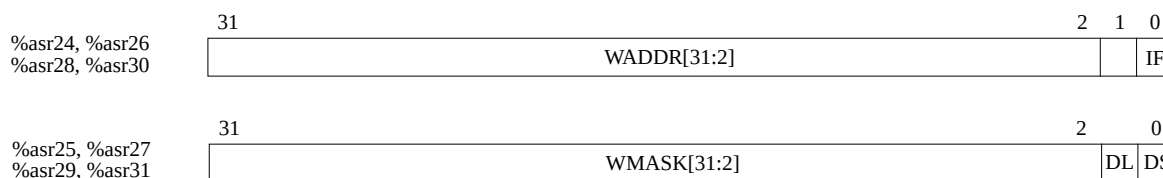
Figure 181. Watch-point registers
