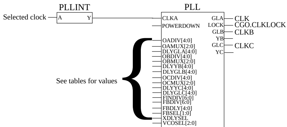
Figure 48. Actel ProASIC3 clock generation
