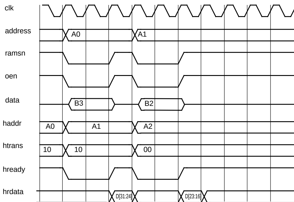
Figure 129. 8-bit SRAM non-sequential read access with 0 wait-states and EDAC enabled.
