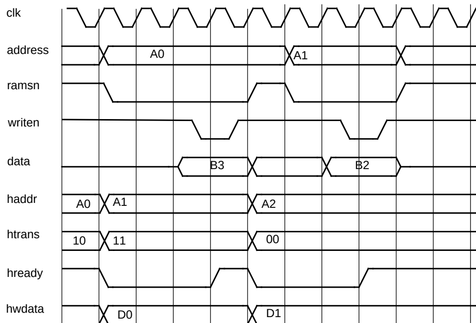
Figure 128. 8-bit SRAM non-sequential write access with 0 wait-states and EDAC enabled.
