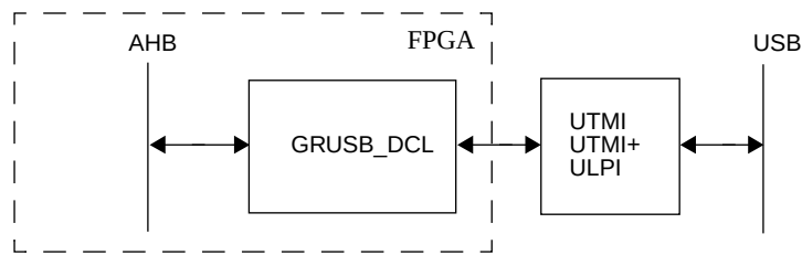
Figure 279. USBDC connected to an external UTM.
