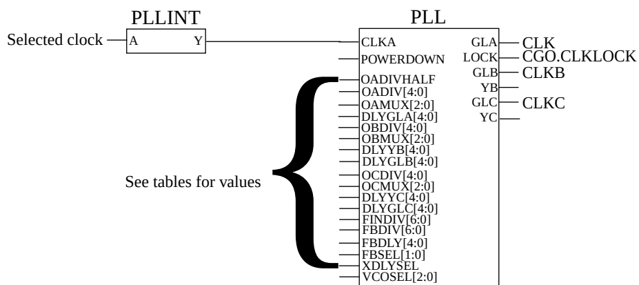
Figure 72. Actel Fusion clock generation
