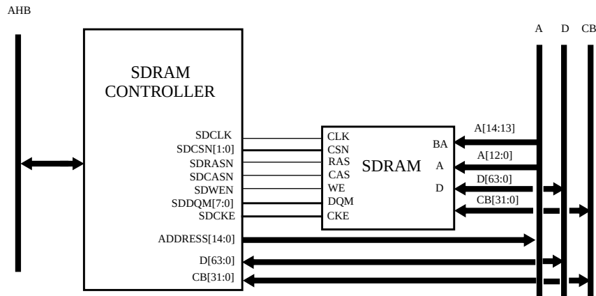
Figure 110. SDRAM Memory controller connected to AMBA bus and SDRAM
