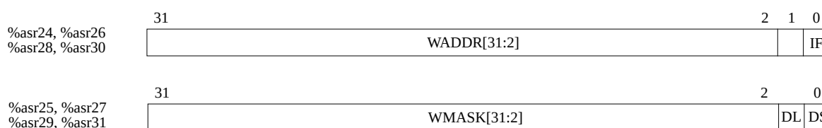
Figure 196. Watch-point registers
