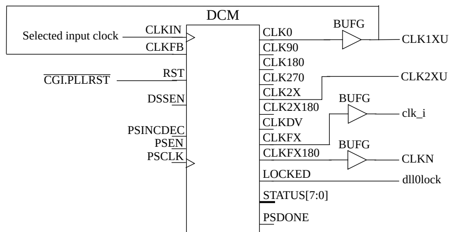
Figure 67. Virtex 5 generation of main clock
