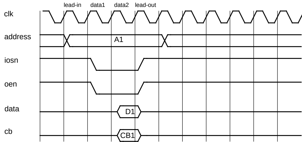
Figure 218. I/O read cycle (0-waitstates)
