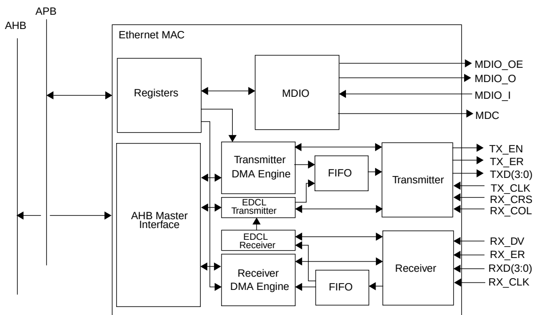
Figure 139. Block diagram of the internal structure of the GRETH.
