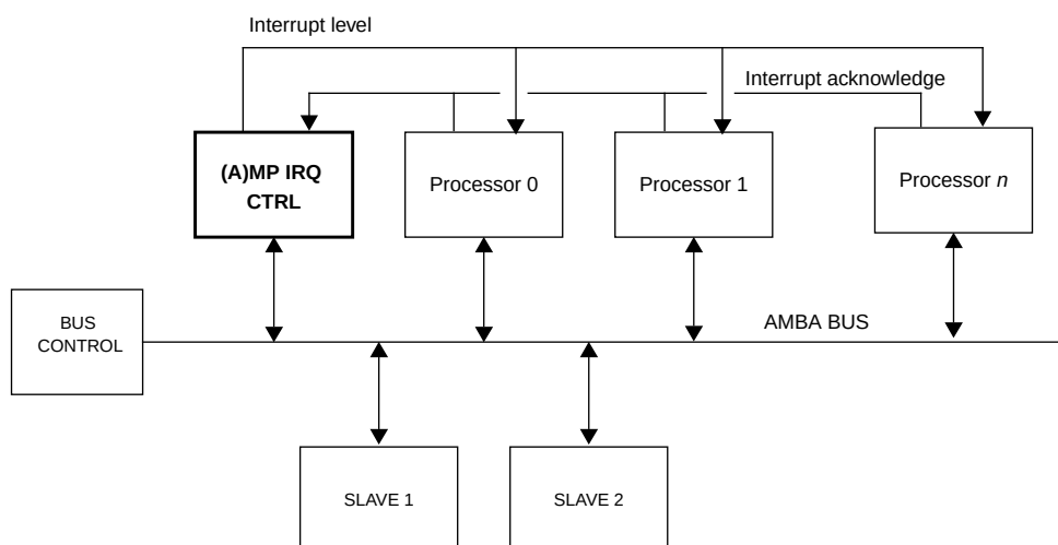
Figure 176. LEON multiprocessor system with Multiprocessor Interrupt controller
