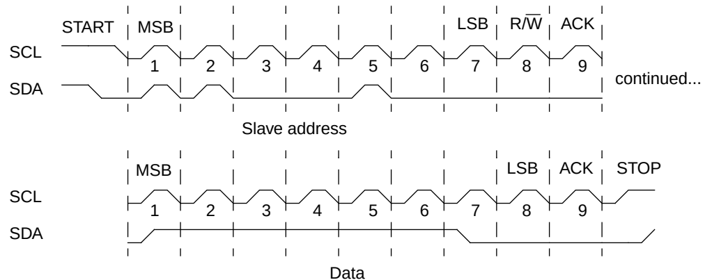
Figure 173. Complete I 2 C data transfer
