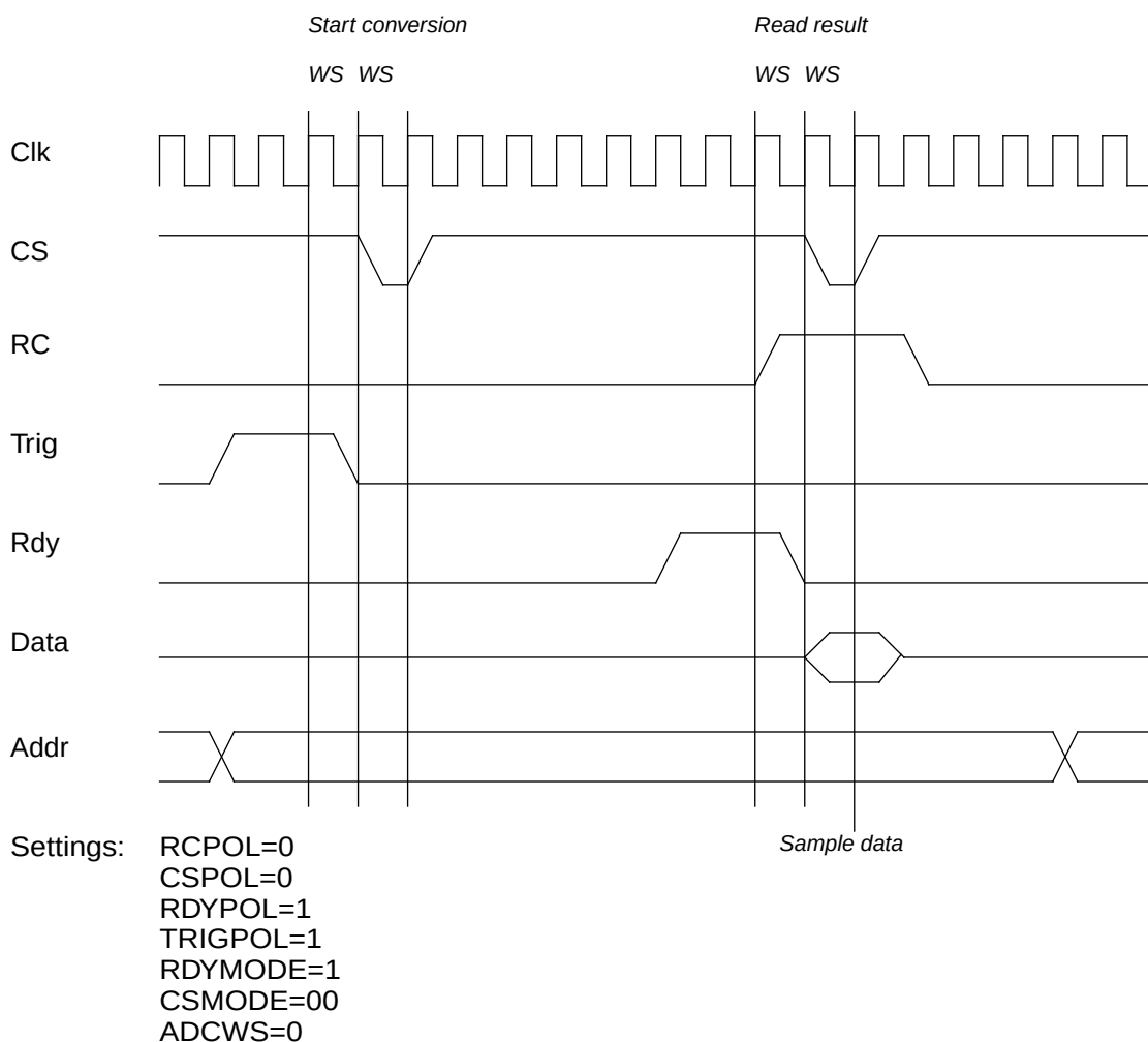
Figure 146. Analogue to digital conversion waveform, 0 wait states (WS)
