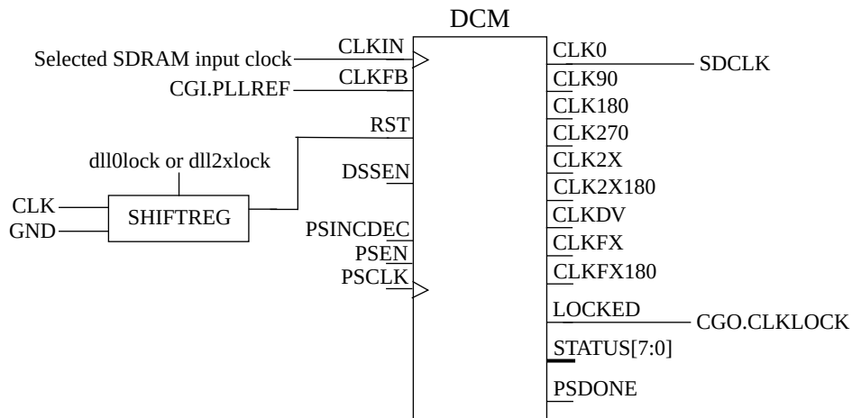
Figure 56. Spartan 3/e generation of SDRAM clock
