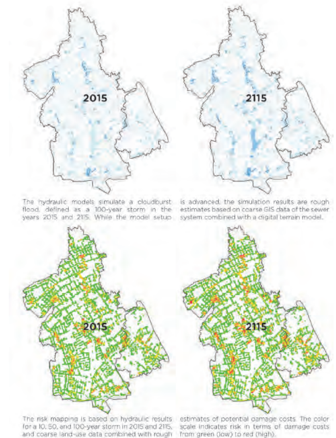
FIGURE 41. NEW YORK CITY URBAN FLOOD MODELING. SOURCE: NEW YORK CITY DEPARTMENT OF ENVIRONMENTAL PROTECTION, JANUARY 2017. CLOUDBURST RESILIENCY PLANNING STUDY. PREPARED BY RAMBOLL A/S.
